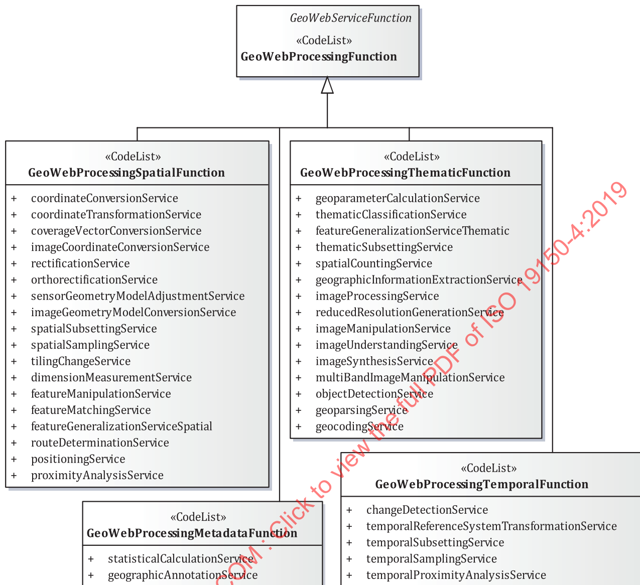
Figure 3 — UML diagram for GeoWeb service processing functions
