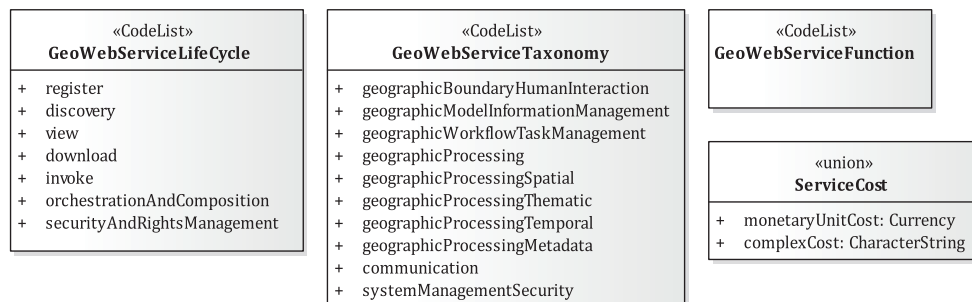
Figure 1 — UML diagram for GeoWeb service identification and description
