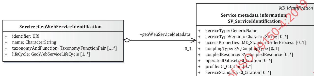
Figure 5 — UML diagram for GeoWeb service metadata
