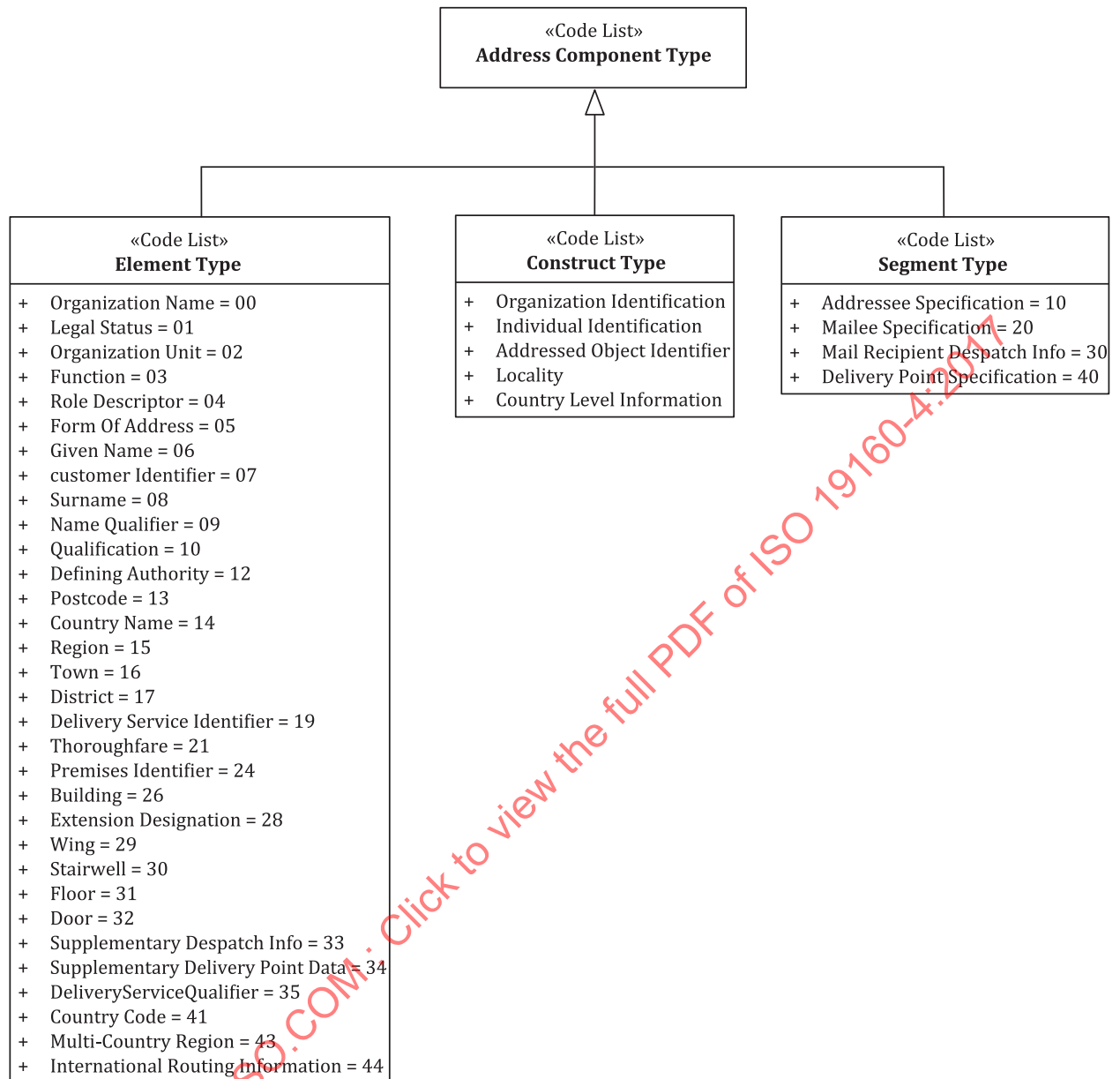
Figure B.10 — Profile code lists
