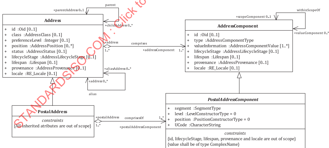
Figure B.1 — Postal address as specialization of ISO 19160-1 address
