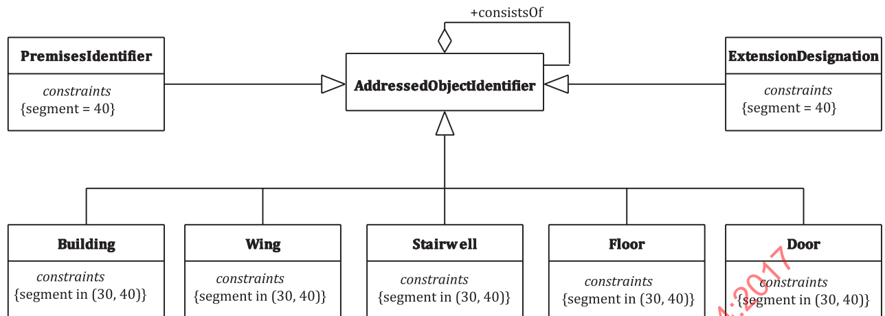
Figure B.7 — Addressed object identifier construct
