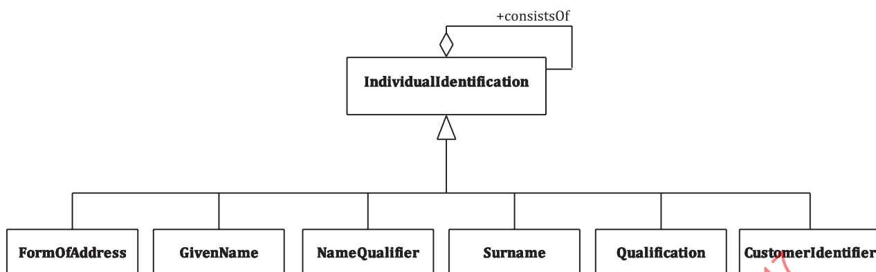
Figure B.3 — Individual identification construct
