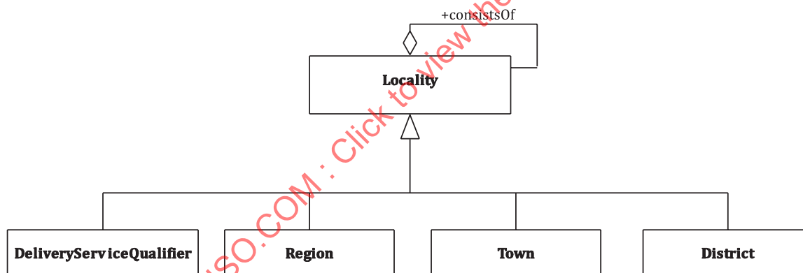
Figure B.6 — Locality construct
