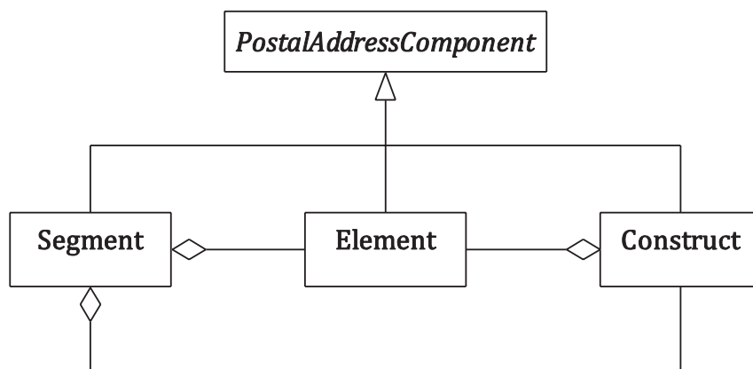
Figure 2 — Relationship between segments, constructs and elements — UML view
