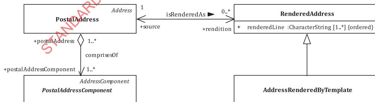
Figure 4 — Rendering of postal address
