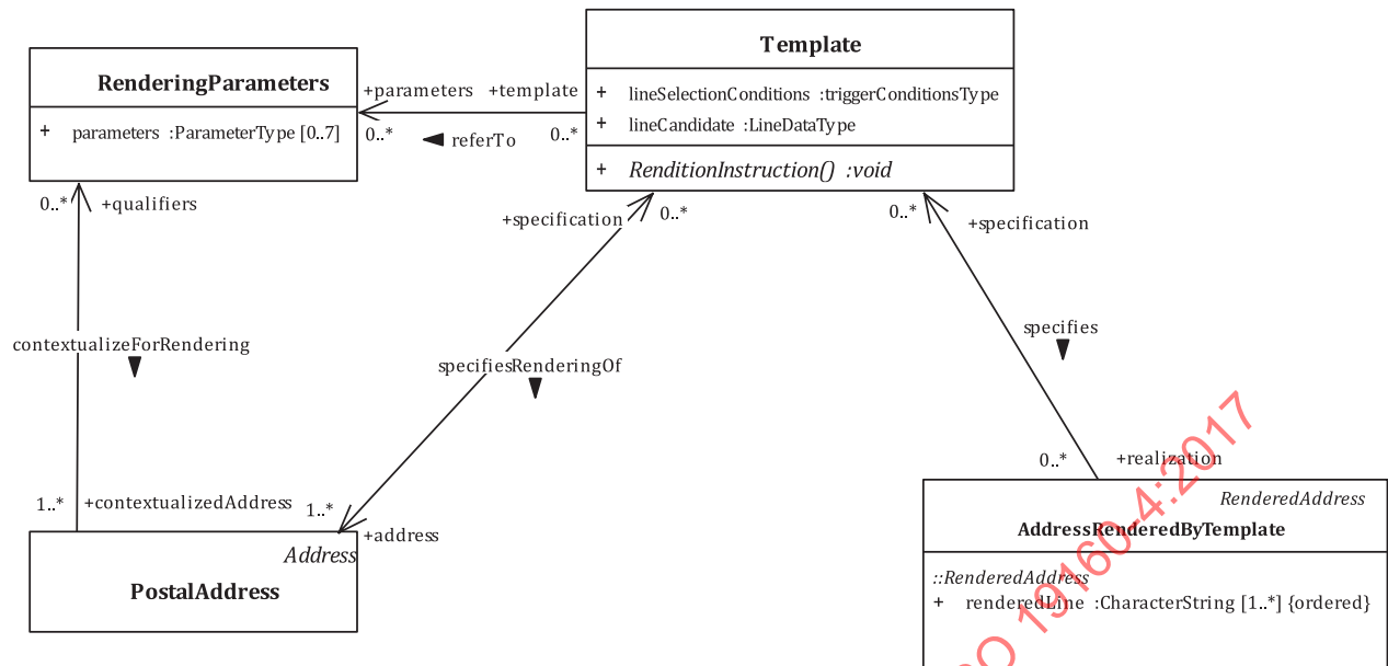
Figure 5 — Rendering of address specified by template
