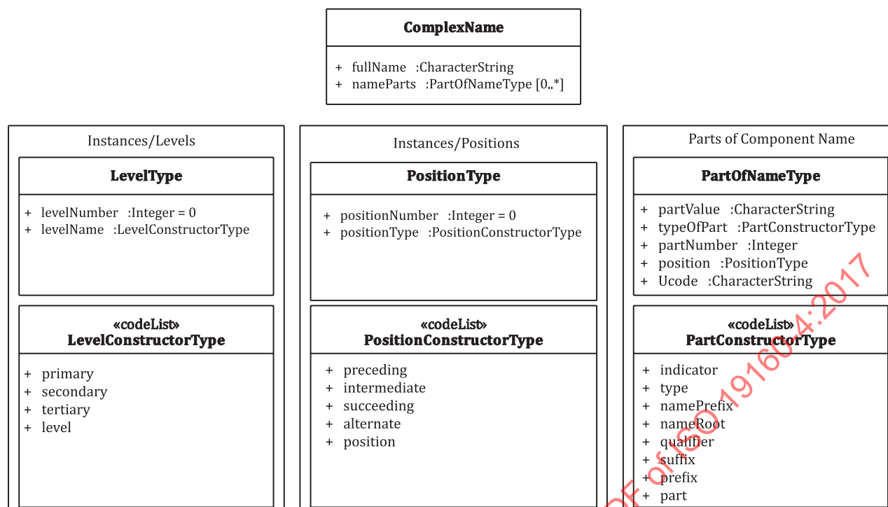
Figure B.9 — Classes supporting sub-elements
