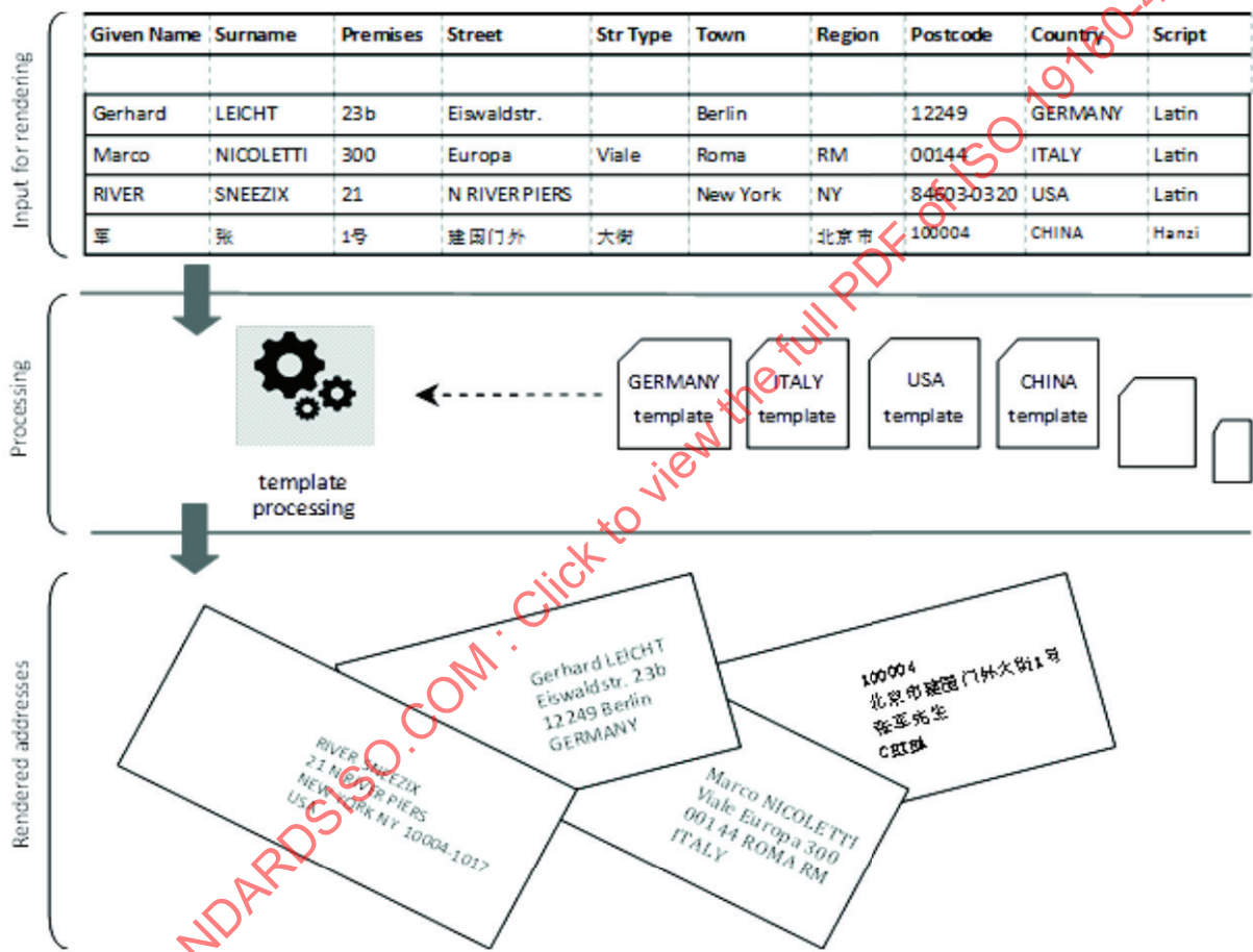
Figure 6 — Automation of postal address rendering with templates
