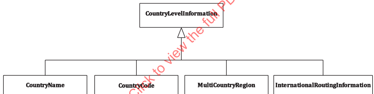
Figure B.8 — Country level information construct
