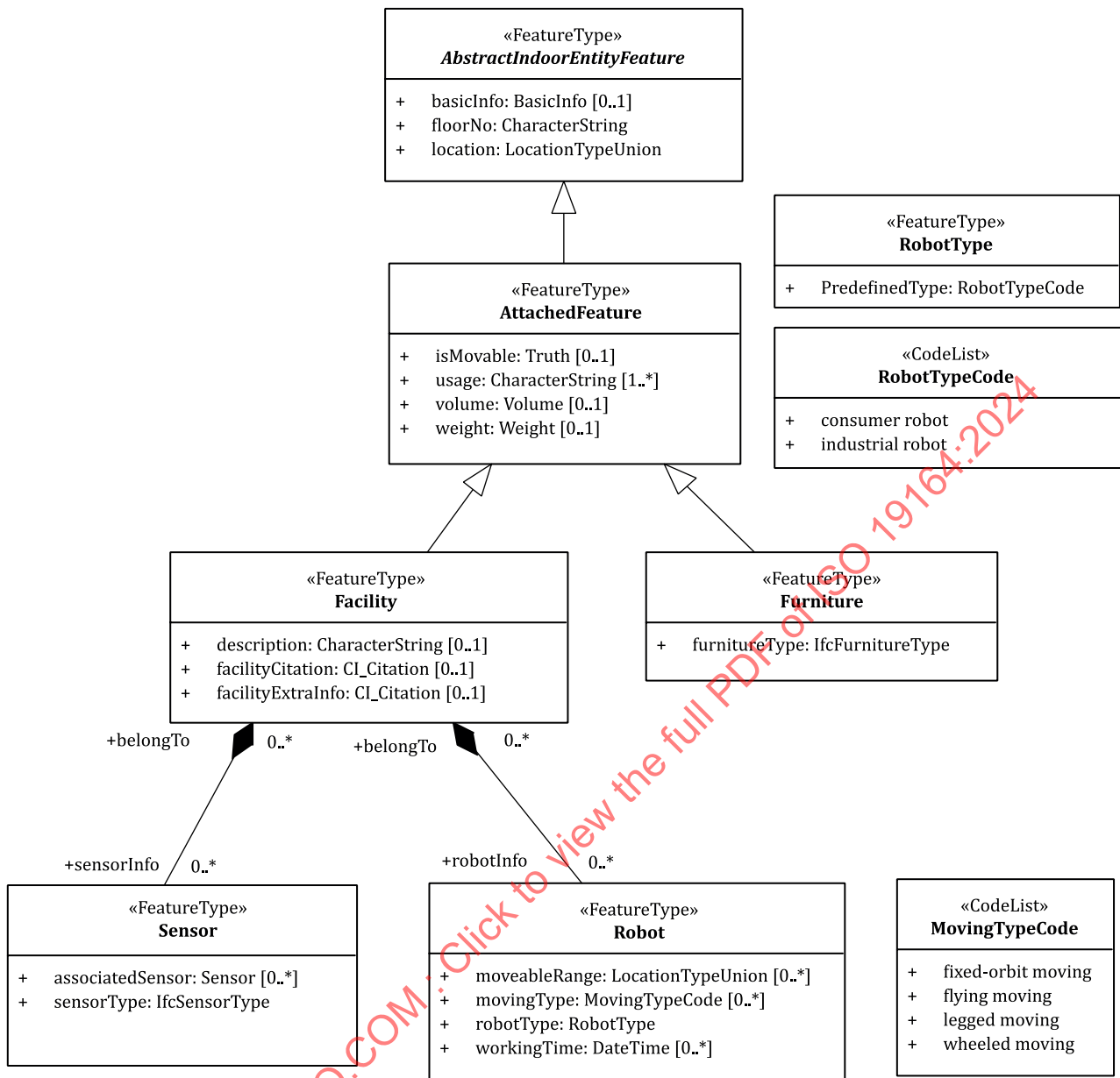
Figure 8 — AttachedFeature class and subclasses
