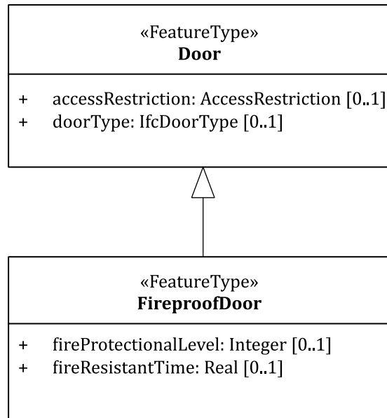
Figure 9 — Example for subclass extension
