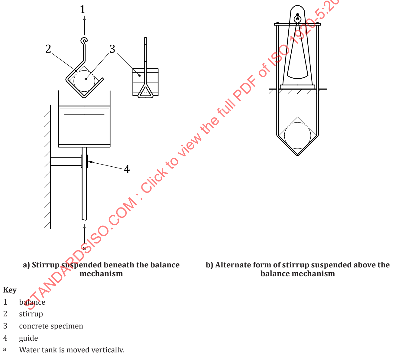
Figure 1 — Typical stirrup arrangement for the determination of the volume of concrete specimens by water displacement
