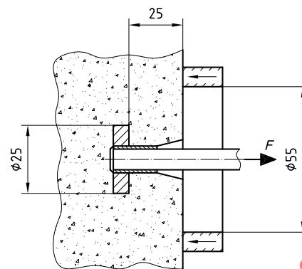
b) Insert installed after casting
