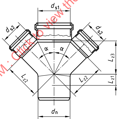
Figure 17 — Double branch
