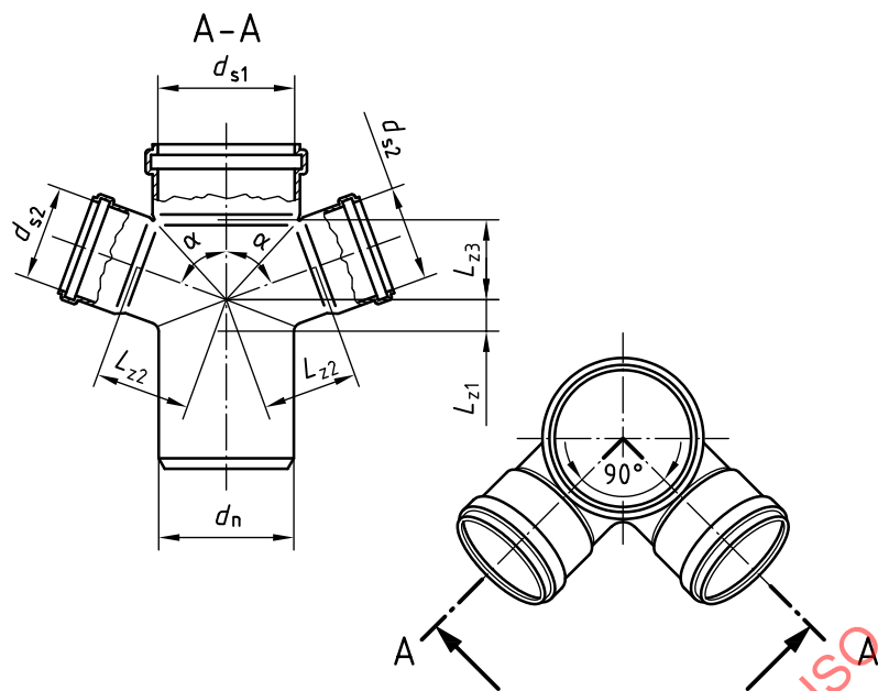
Figure 18 — Angular double branch
