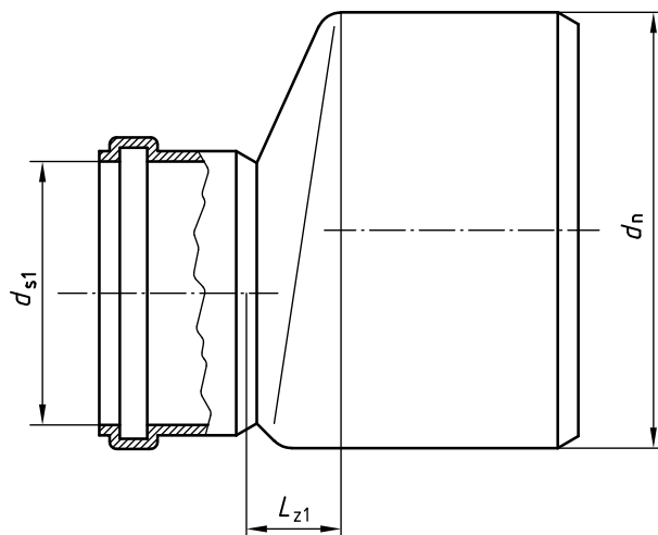
Figure 20 — Reducer
