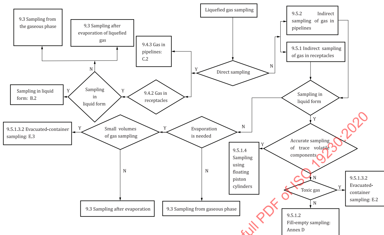
Figure 8 — Block diagram of liquefied gas sampling method
