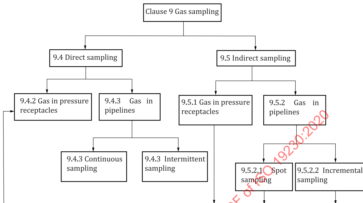
Figure 2 — Gas sampling classification
