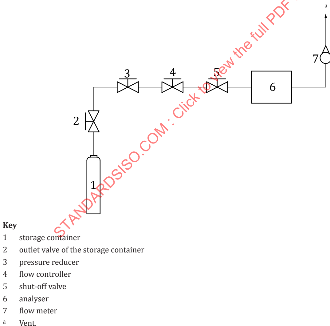
Figure B.2 — Flow chart of direct sampling without a vacuum pump for gas in pressure receptacles
