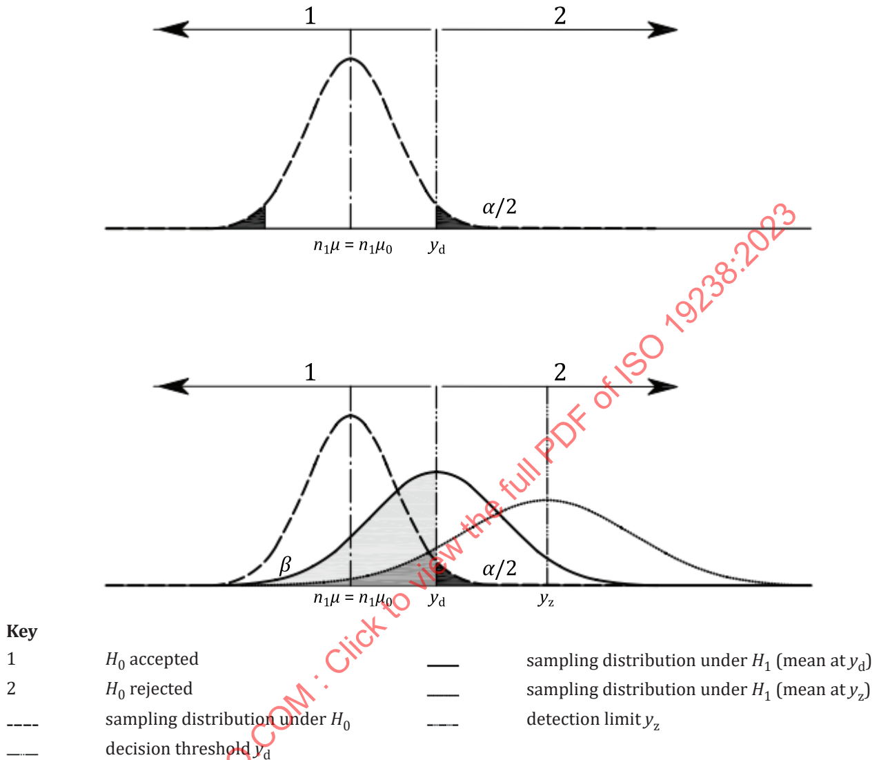
Figure 1 — Illustration of the decision threshold and the detection limit ( \mu_0 = \text{const} )
