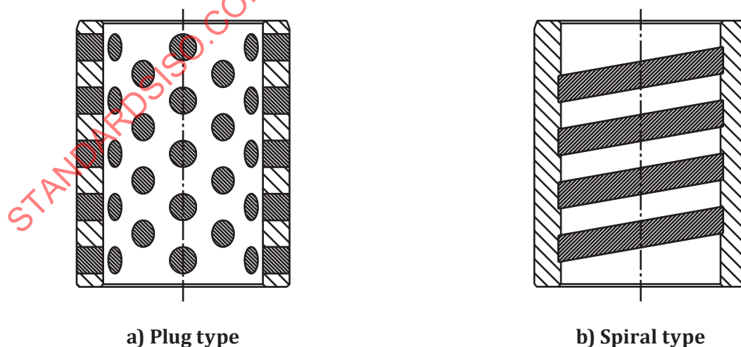
Figure 1 — Embedded state of solid lubricants on cylindrical bush
