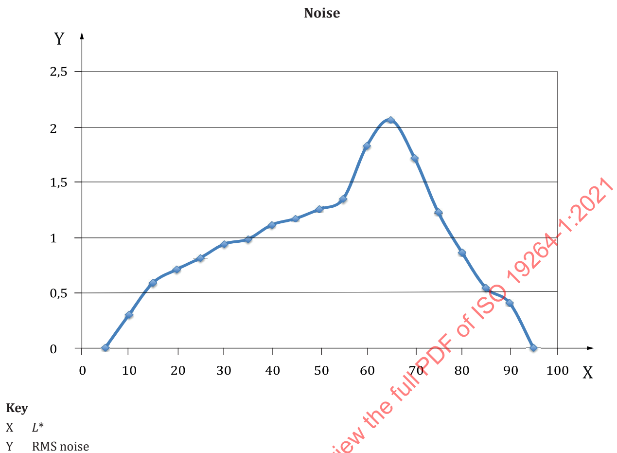
Figure 4 — Graphical presentation of RMS noise over the L^* value of the grey scale
