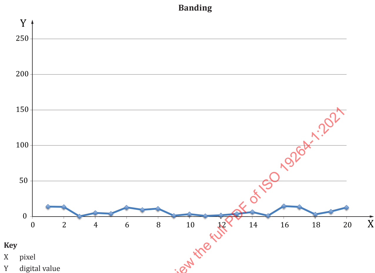
Figure 5 — Digital values over pixels (Regular peaks in this structure indicate the presence of banding in images)
