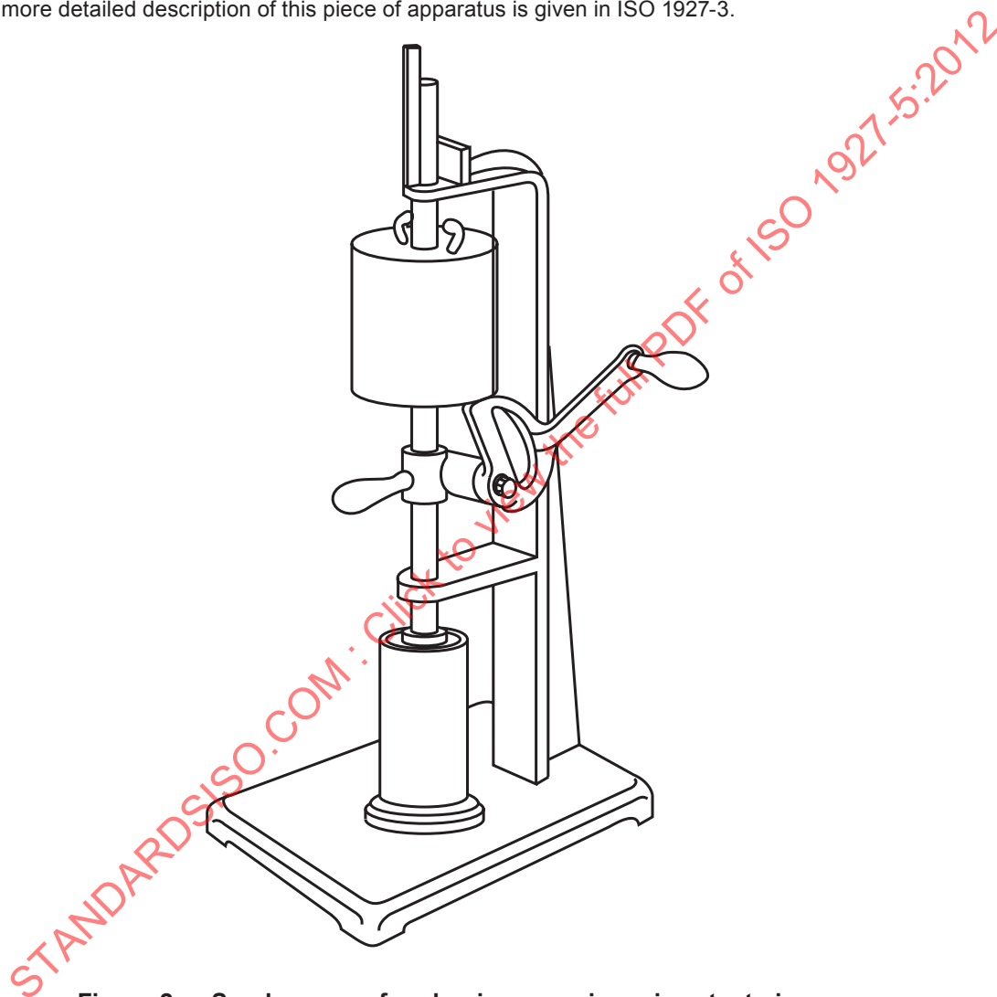
Figure 2 — Sand-rammer for shaping ramming mixes test pieces
