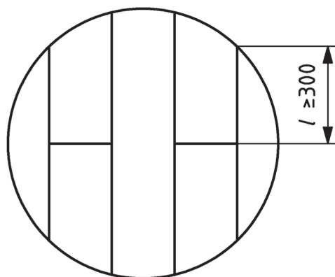
Figure 1 — Example of an assembled test area for a castor chair test (planks)
