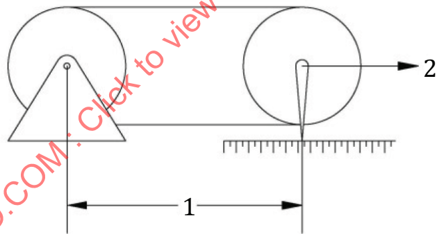
Figure 4 — Clearance between measuring pulley and belt
