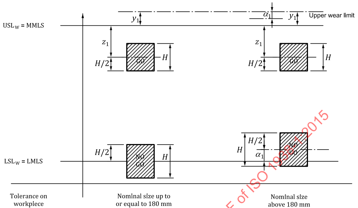
Figure 3 — MPL size position for GO and NO GO gauges for workpieces for an external feature of size
