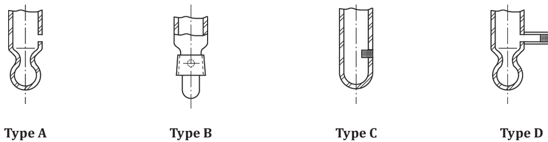
Figure 4 — pH electrodes
