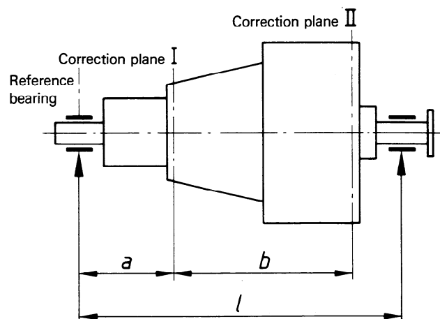
Figure 6 — Rotor dimensions to be used for general method calculations
