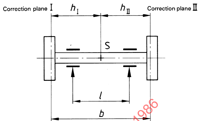
Figure 4 — Rotor with overhung discs at both ends
