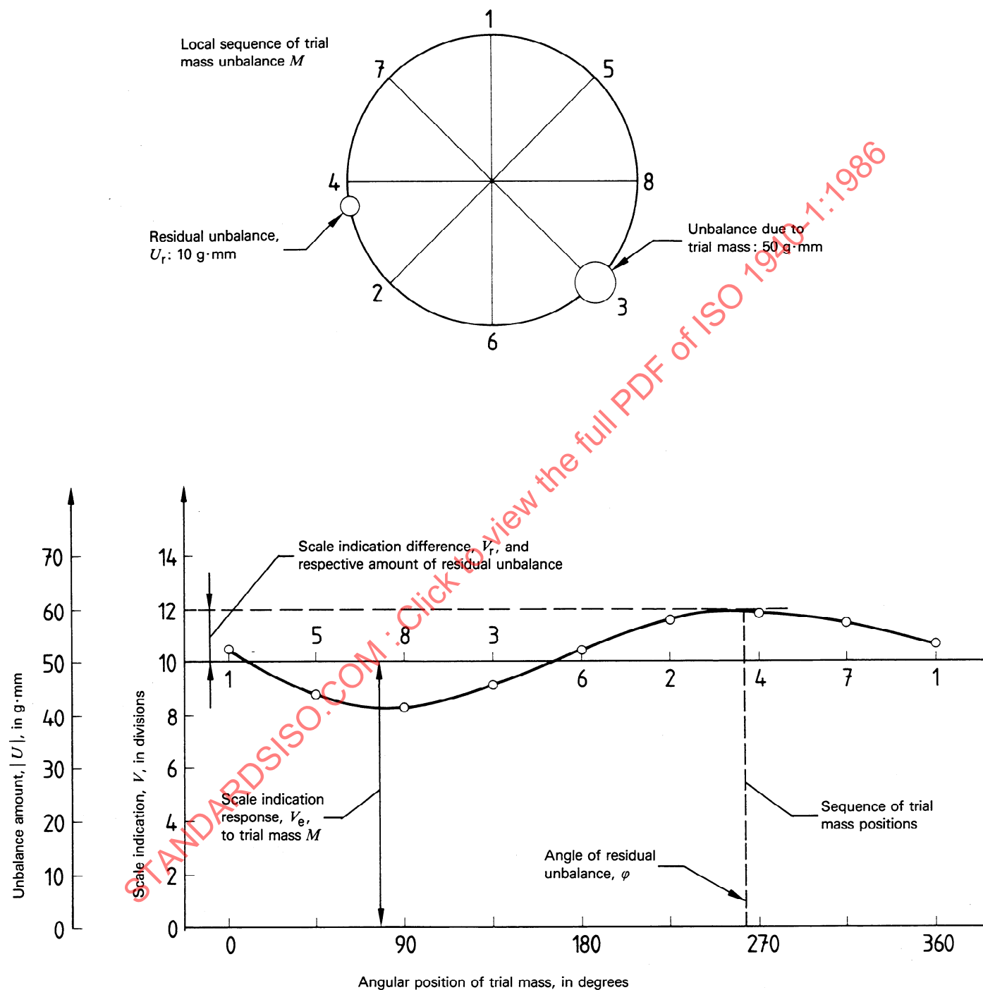
Figure 8 — Test procedure for determining the residual unbalance in one plane
