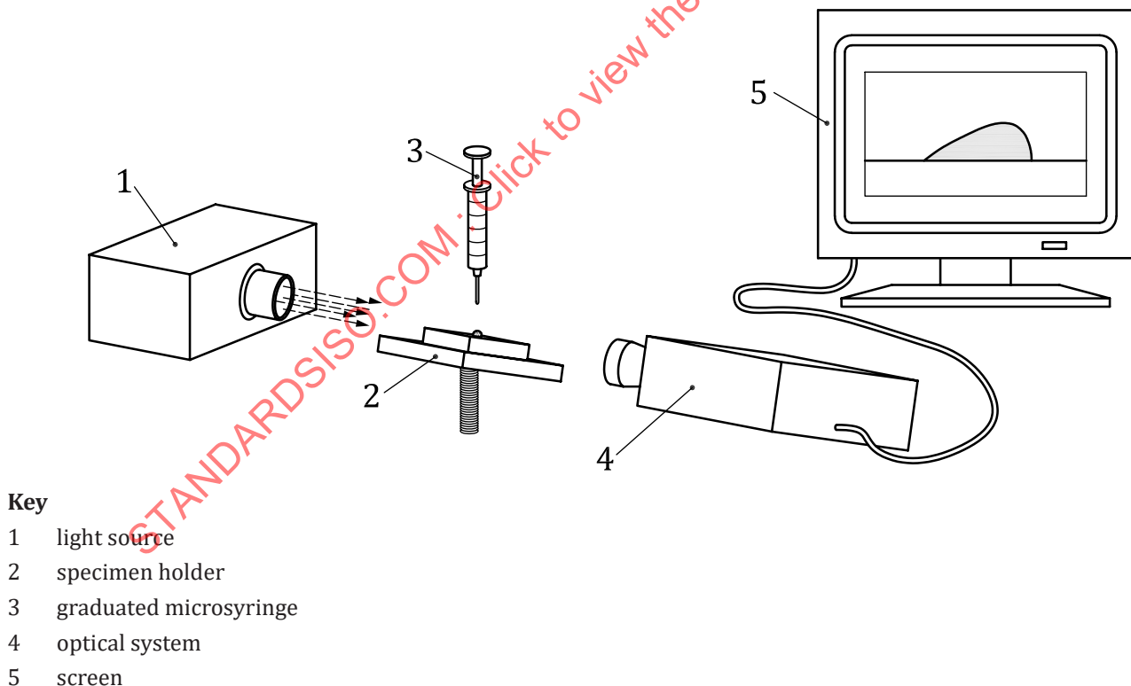
Figure 1 — Schematic diagram of a contact angle measuring system for which the camera as well as the sample table are inclined
