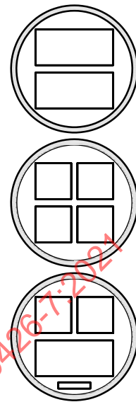
Figure B.1 — Shaft configurations included in the scope of Annexes B to F
