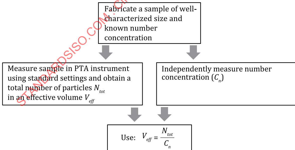
Figure 3 — Schematic process flow for estimation of effective sampling volume
