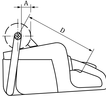
Figure 3 — Clearance and distance between front and rear handles for rear handle machines
