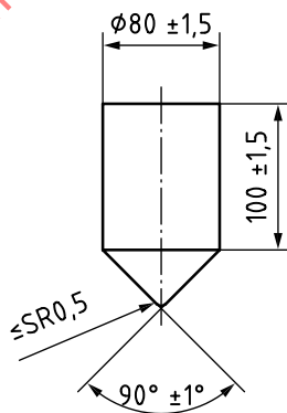
Figure 13 — Test cone
