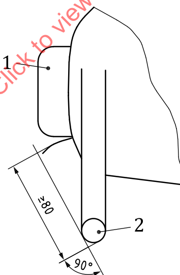
Figure 10 — Required distance between front handle and unprotected hot part
