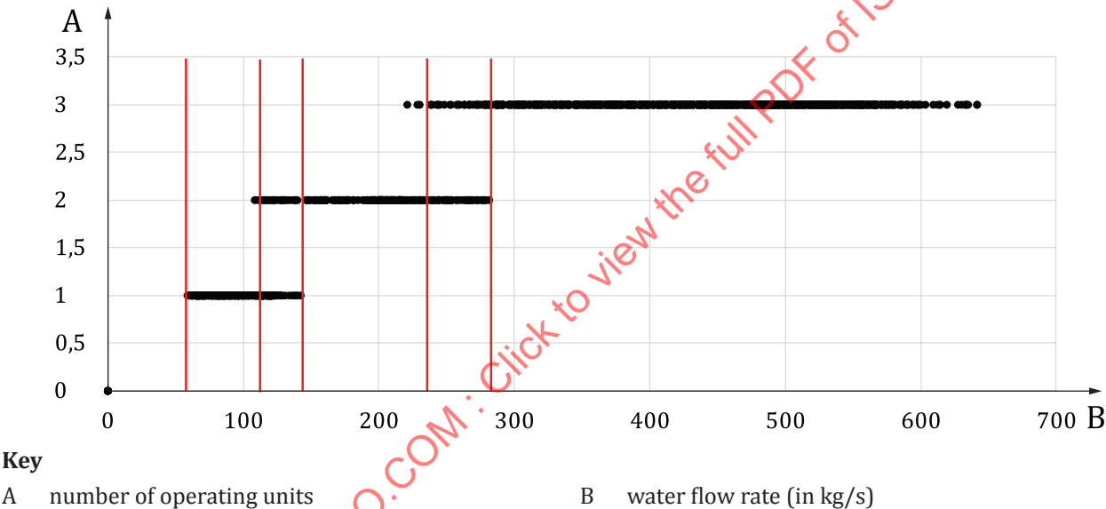
Figure 6 — Example of the relationship between water flow rate and number of operation units
