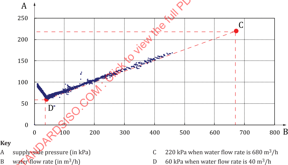
Figure 7 — Example of the relationship between water flow rate and pressure (control system type B)
