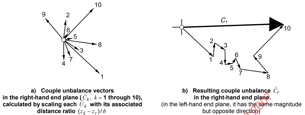
Figure A.6 — Graphical representation and evaluation of unbalances, resultant couple unbalance
