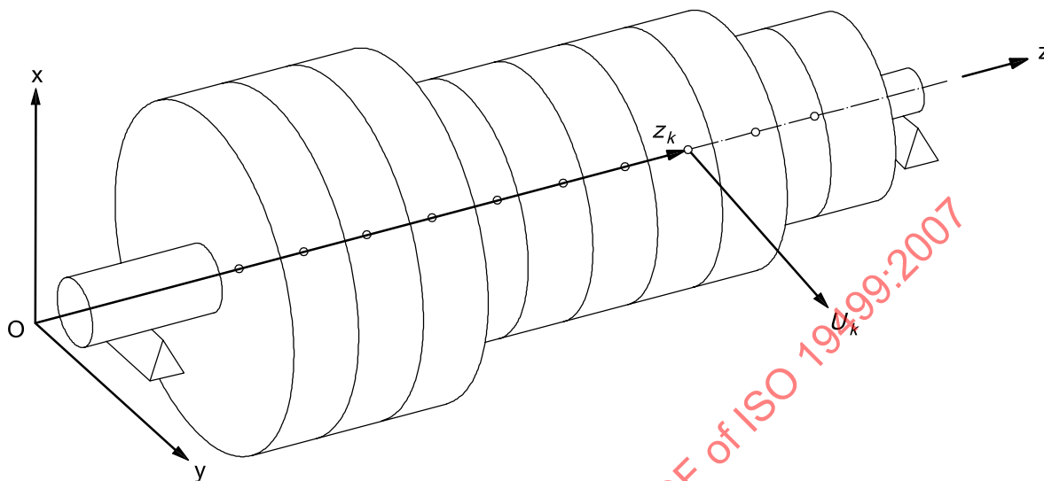
Figure A.2 — Unbalance vector \vec{U}_k at axial position \vec{z}_k
