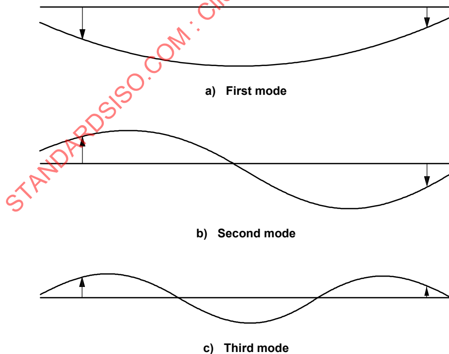
Figure 3 — Schematic representation of the first three flexural modes of a rotor with flexible behaviour on an elastic support structure
