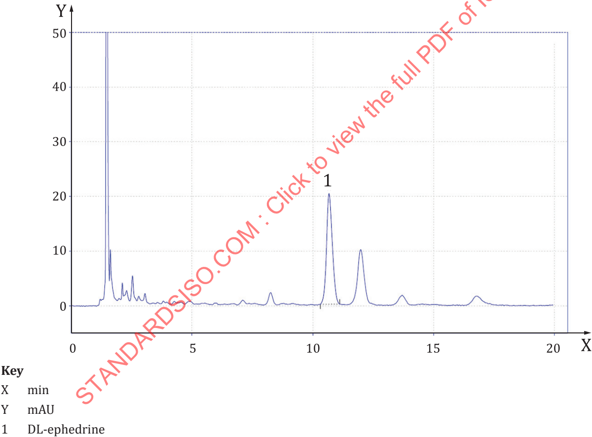
Figure B.3 — Typical chromatogram of Ephedra Herba
