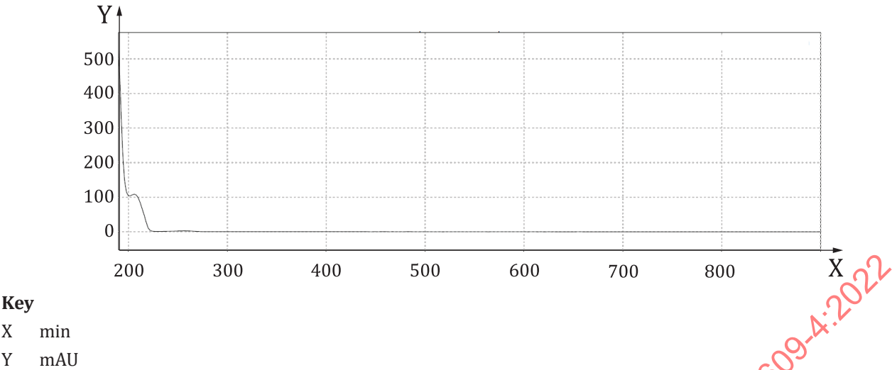
Figure B.2 — Typical UV-vis spectrum of DL-ephedrine
