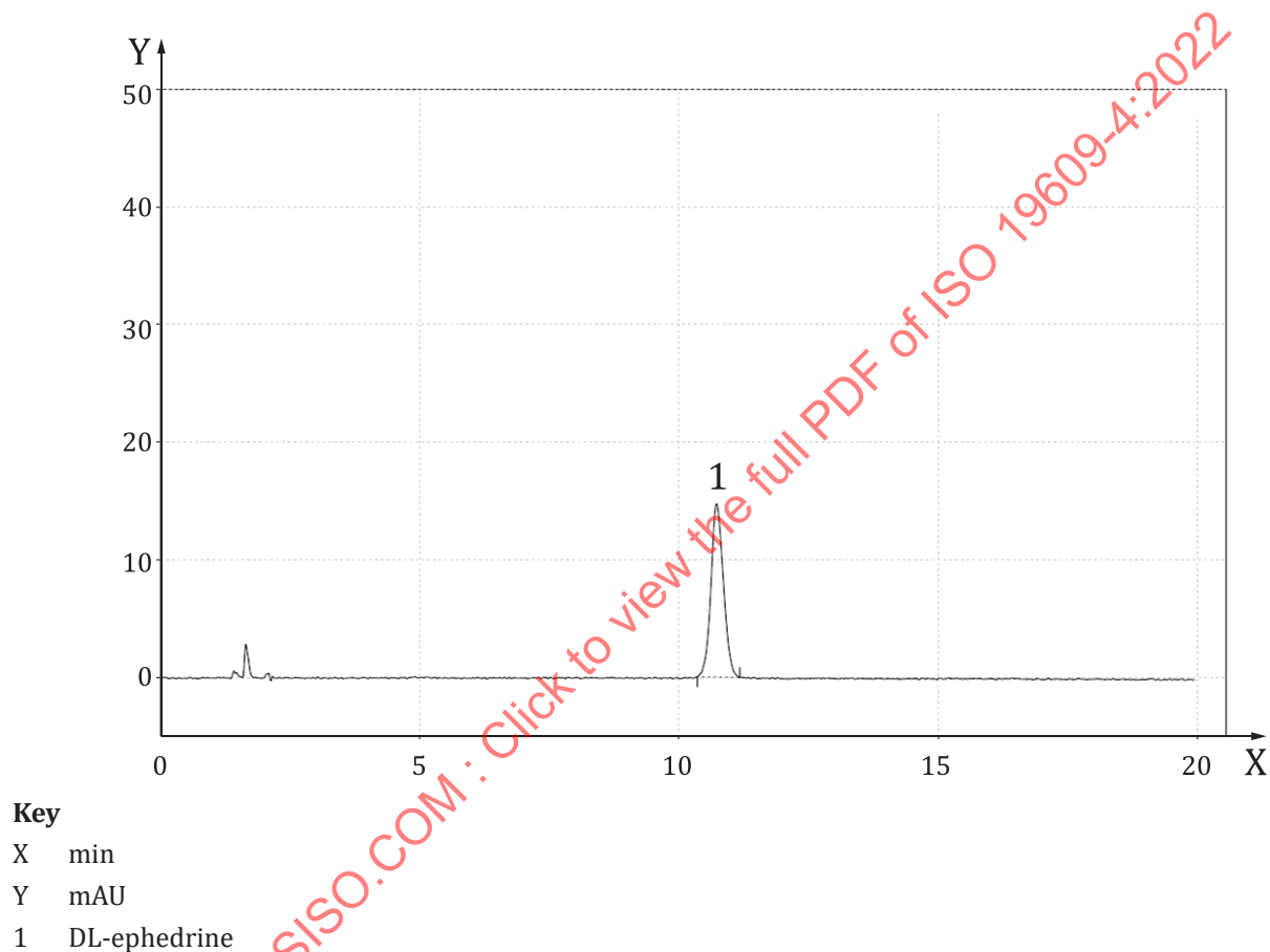
Figure B.1 — Typical chromatogram of DL-ephedrine standard
