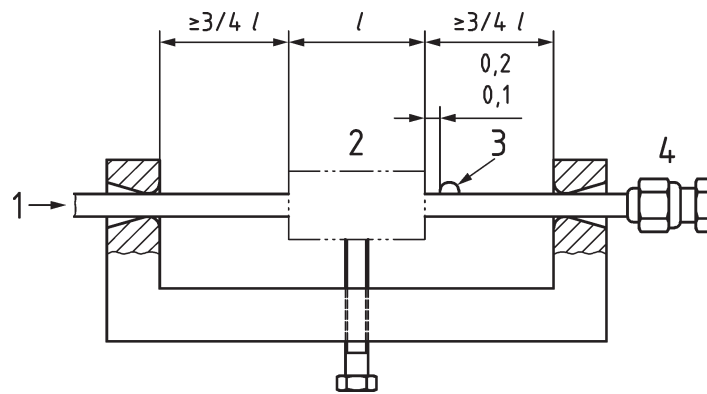
a) Straight fitting test setup
