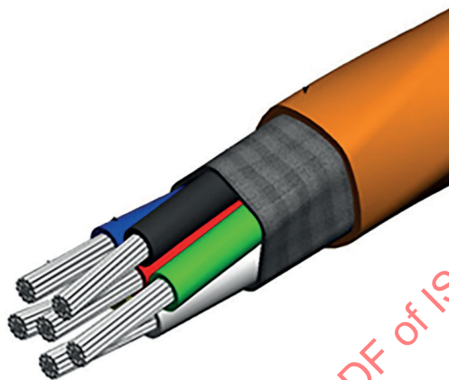
Figure 6 — Multi-core cable with screen and sheath
