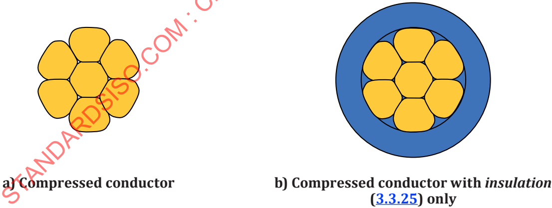
Figure 3 — Compressed conductor
