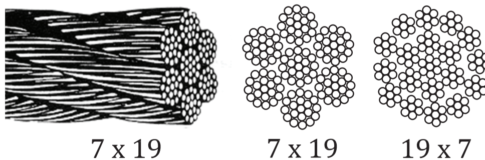
Figure 7 — Rope-stranded conductors
