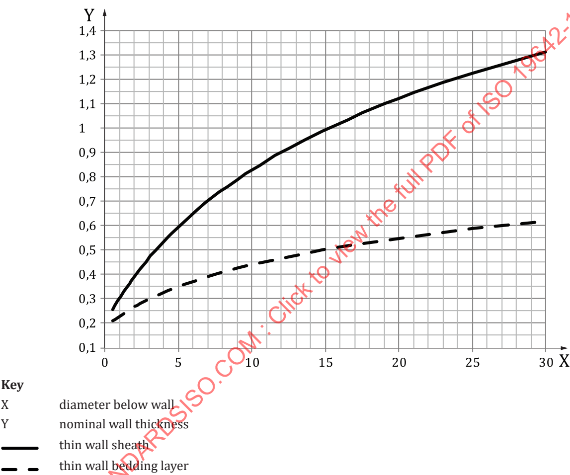
Figure A.3 — Wall thicknesses for thin wall constructions
