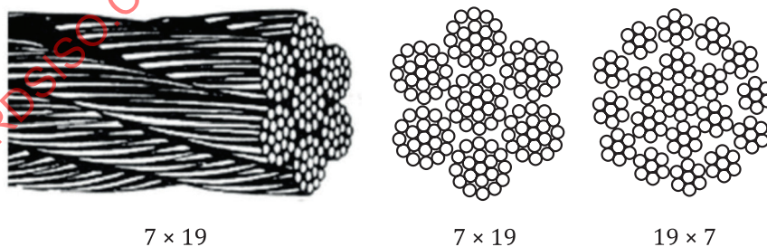
Figure 7 — Rope-stranded conductors
