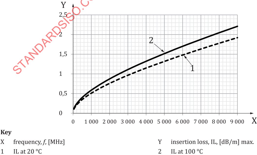
Figure 11 — CX44c, insertion loss limit
