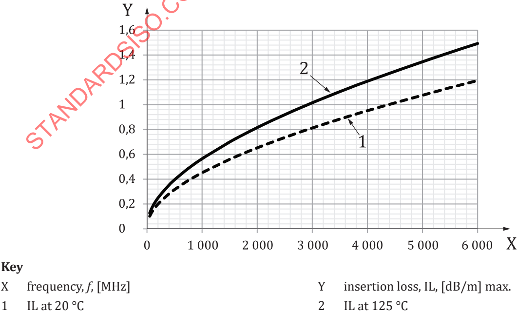
Figure 8 — CX58c, insertion loss limit
