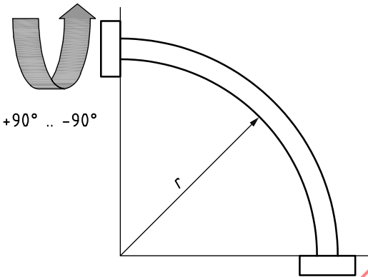
Figure 26 — Torsion test rig
