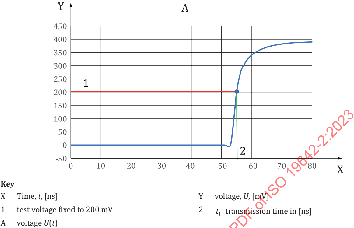
Figure 24 — Delay time readout
