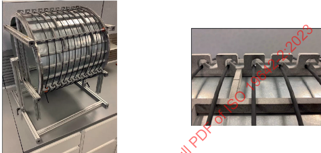
Figure 18 — Test set up 3 on metallic drum, alternative
