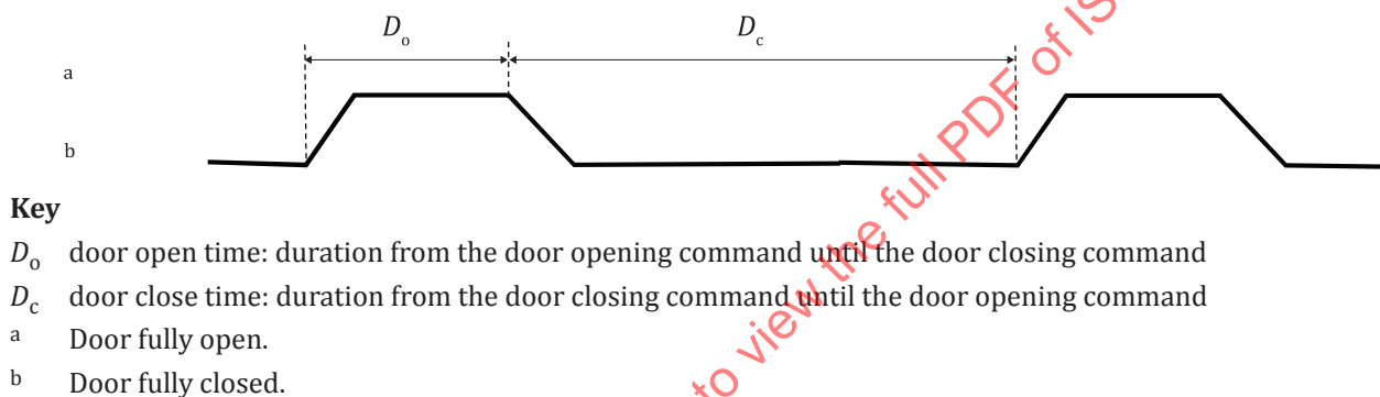
Figure 5 — Explanation of door open and close times
