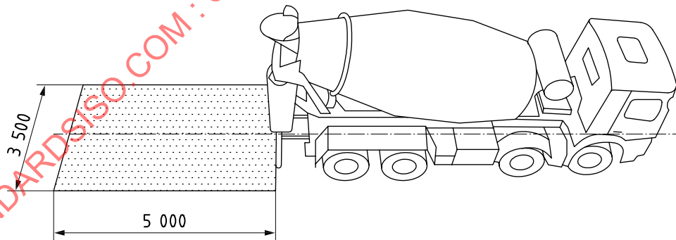
Figure A.16 — Minimum dimensions of the visibility test rectangle (VTR)
