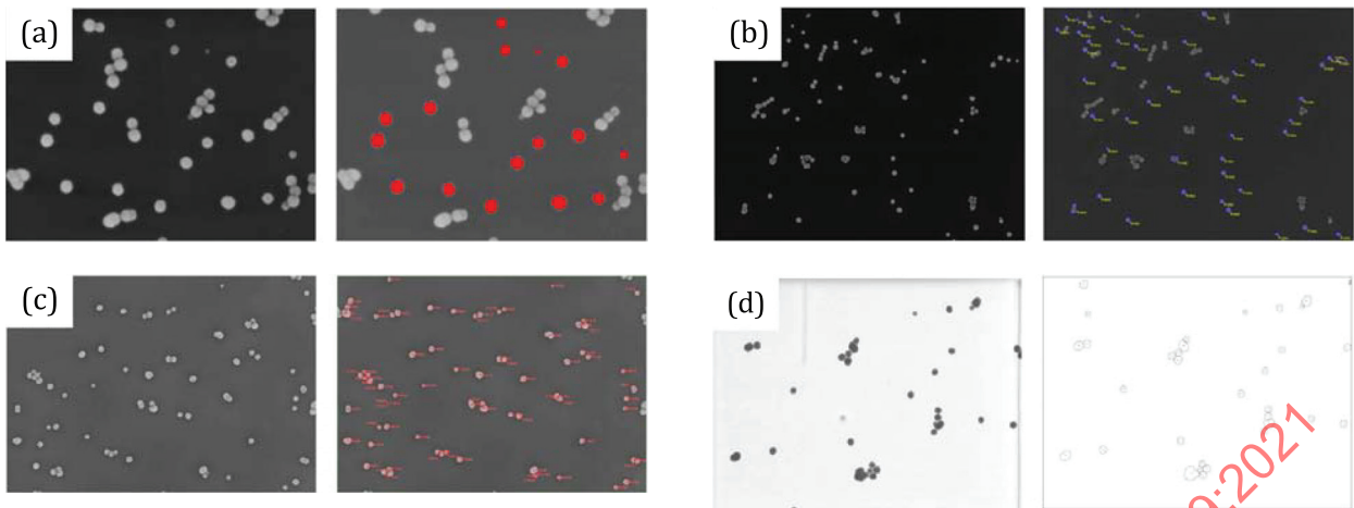
Figure C.3 — Typical SE images (left pane) and analysed images (right pane) in Phase 2, reported by participant A (a), D (b), E (c) and I (d)
