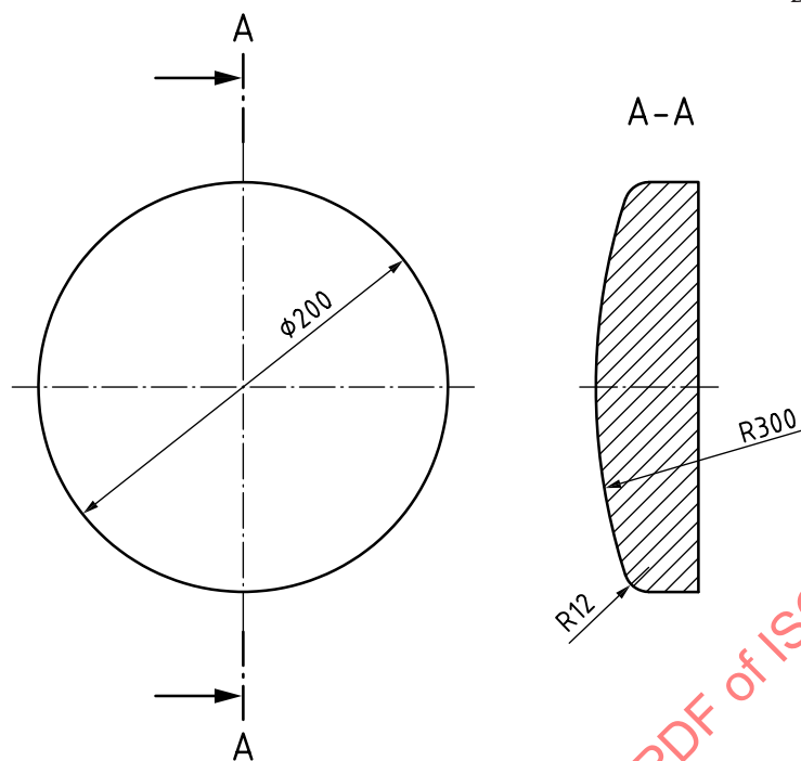
Figure 1 — Loading pad
