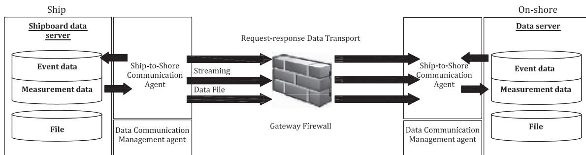
Figure A.2 — Concept model of ship-to-shore communication agent
