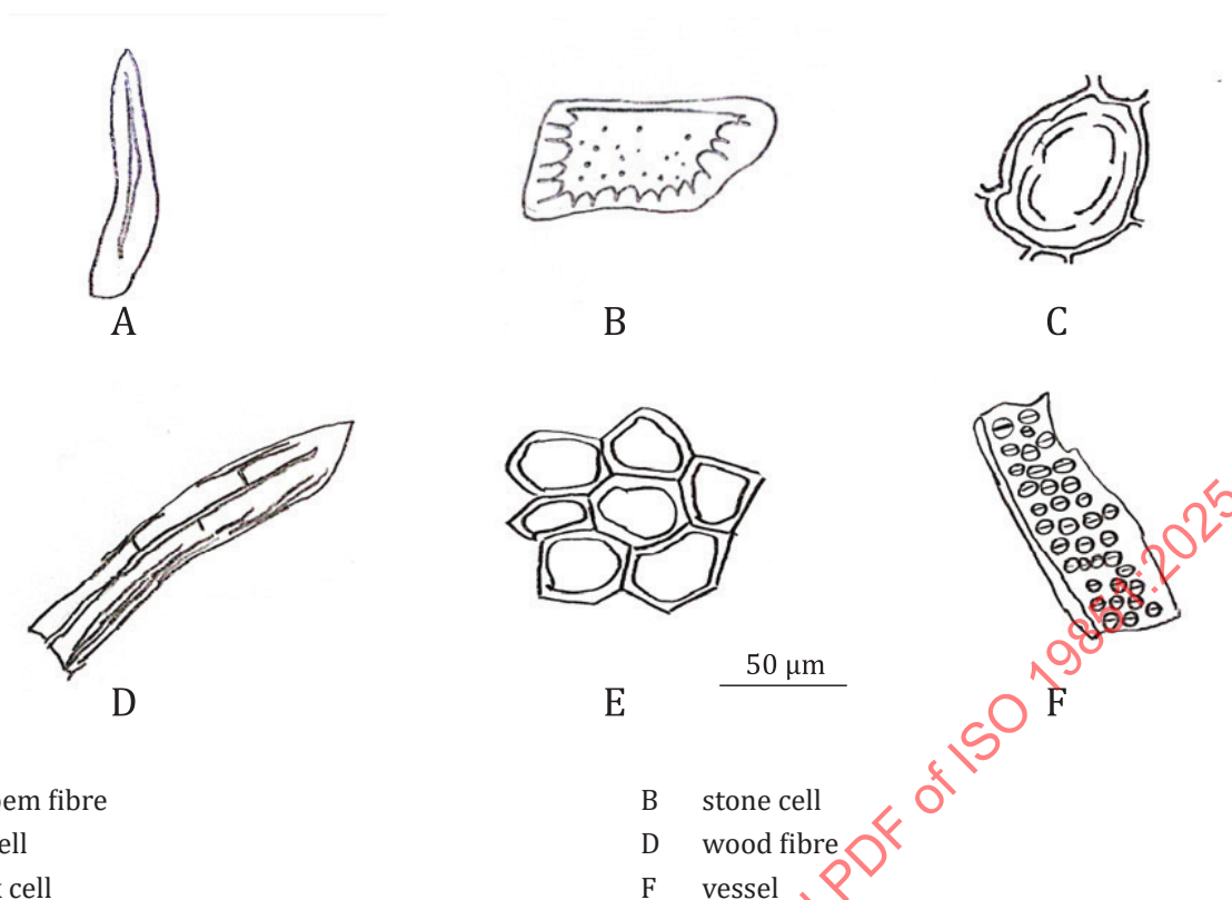
Figure 3 — Microscopic features of the powder of Cinnamomum cassia Presl. (Lauraceae)
