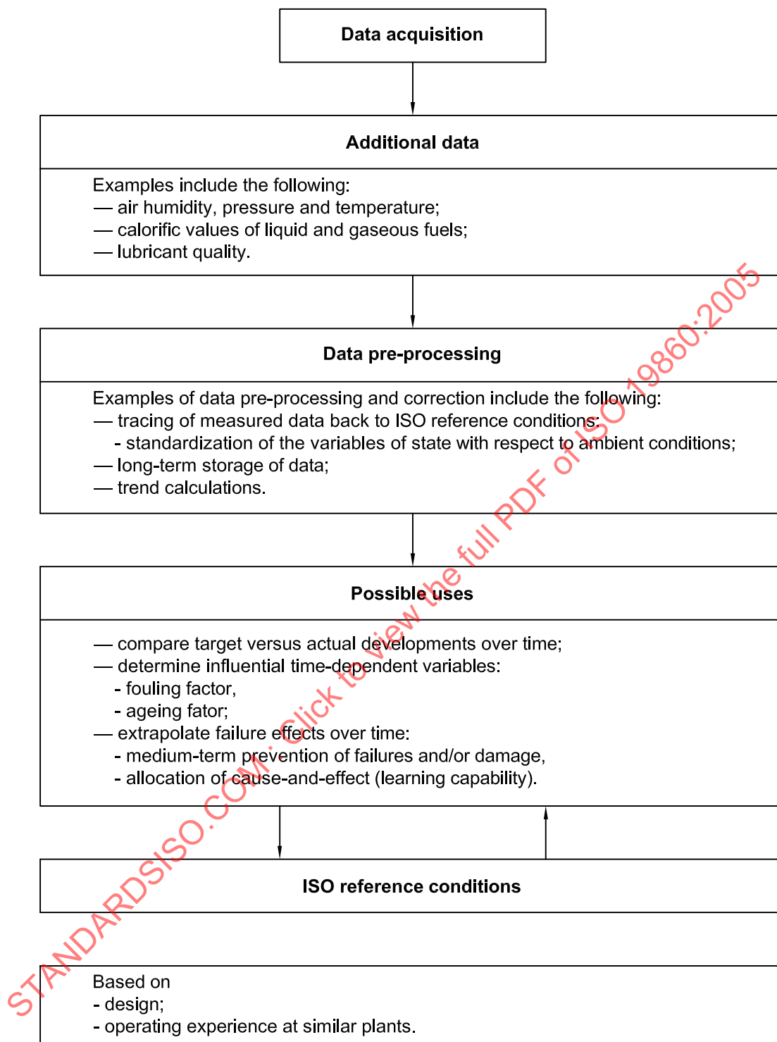
Figure 2 — Trend-monitoring system (TMS)
