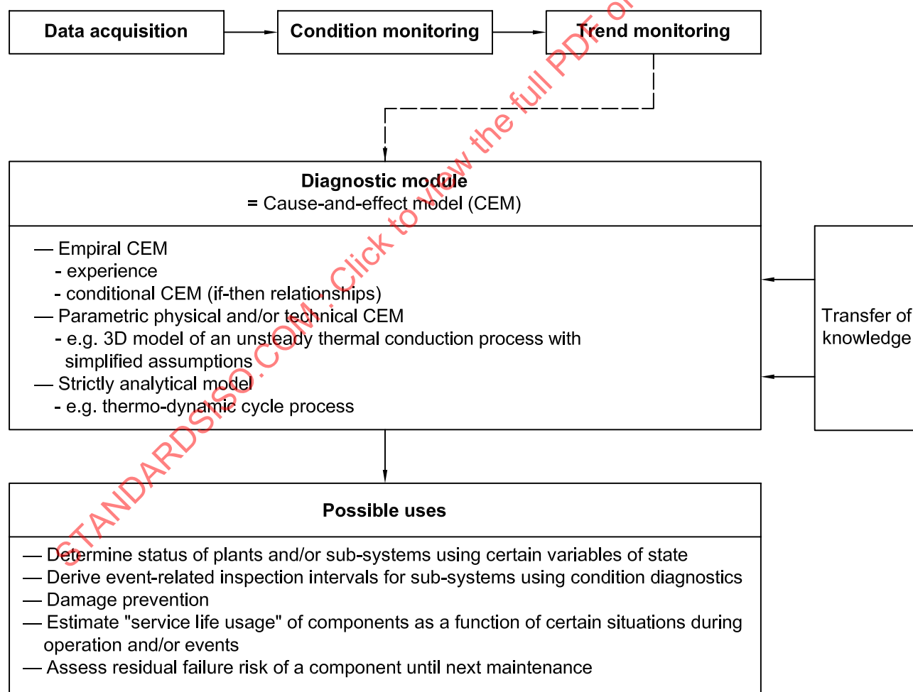
Figure B.1 — Diagnostic systems (DS)
