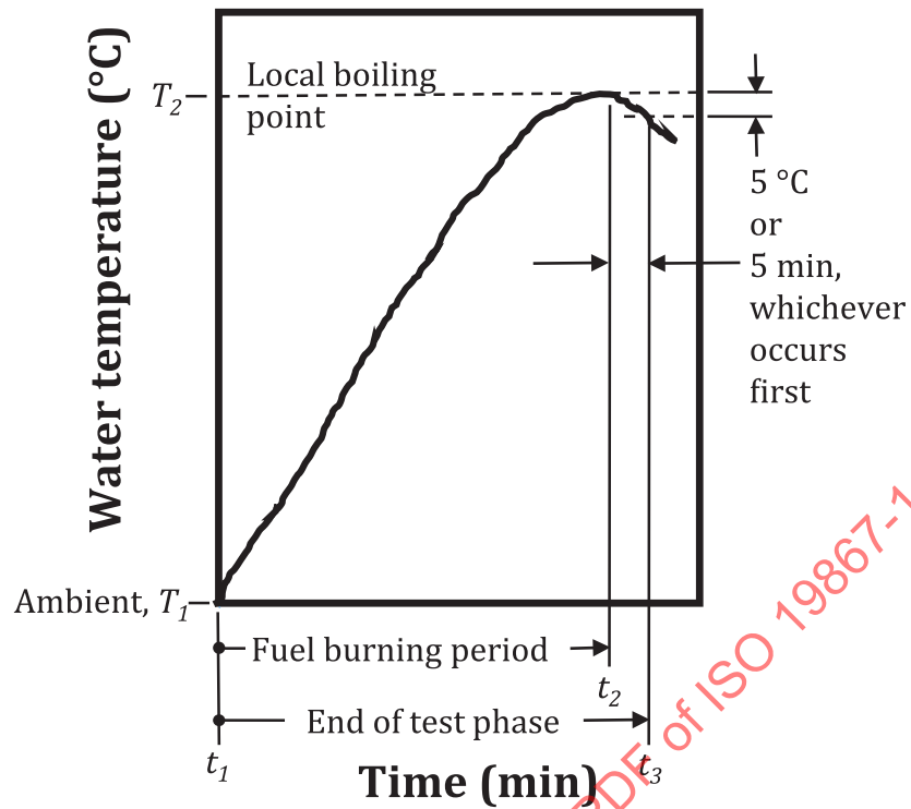
Figure 4 — Illustrative graph of water temperature versus time for any test phase when water temperature reaches the local boiling point at the end of the fuel burning period
