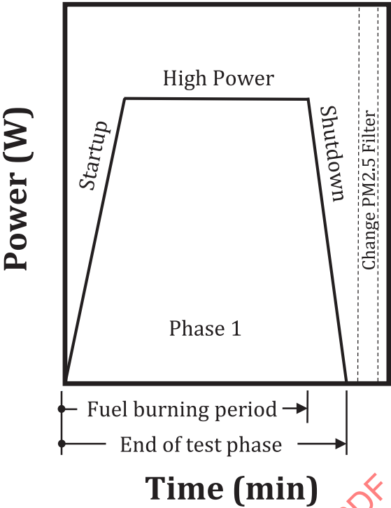
Figure 1 — Diagram of the standard test sequence for cookstoves with a single power level
