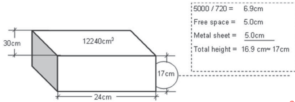
Figure C.7 — Example dimensions of each of two Mylar pots for 40 cm by 60 cm griddle
