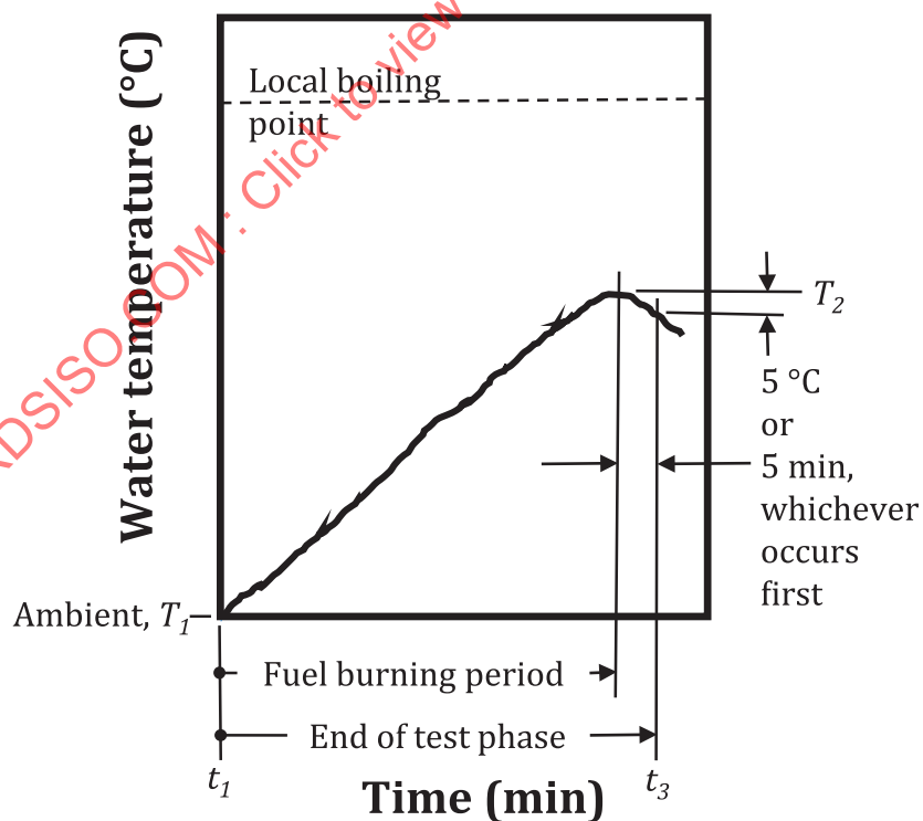
Figure 5 — Illustrative graph of water temperature versus time for any test phase when water temperature does not reach the local boiling point
