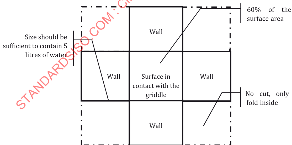
Figure C.1 — Assembly of Mylar pot
