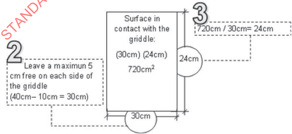
Figure C.6 — Example dimensions of Mylar pot surface for each of two mylar pots in contact with 40 cm by 60 cm griddle
