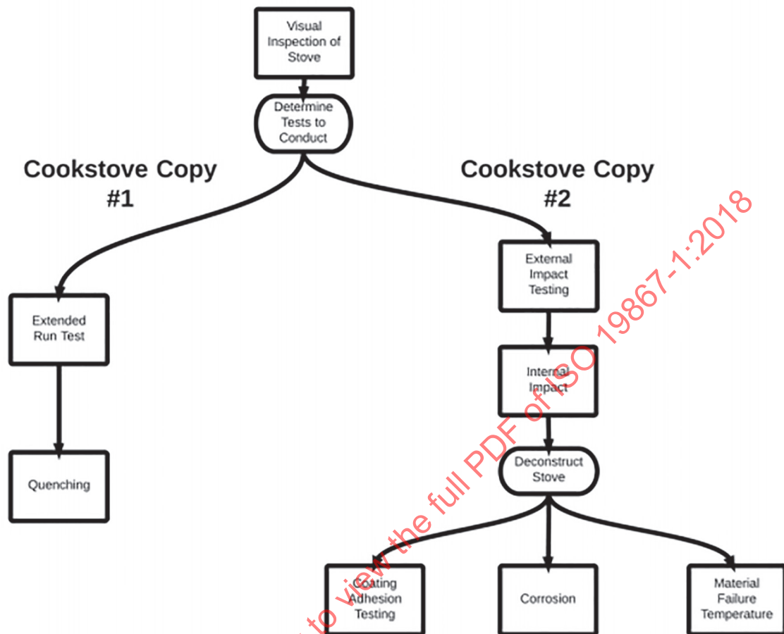
Figure 8 — Sequential order of cookstove durability stress tests
