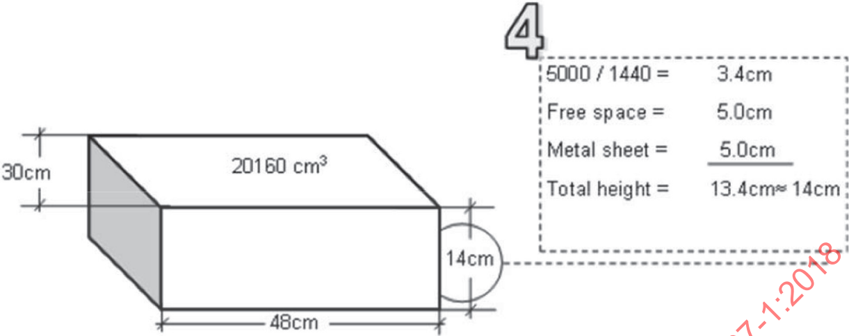
Figure C.4 — Example Mylar pot dimensions for 40 cm by 60 cm griddle
