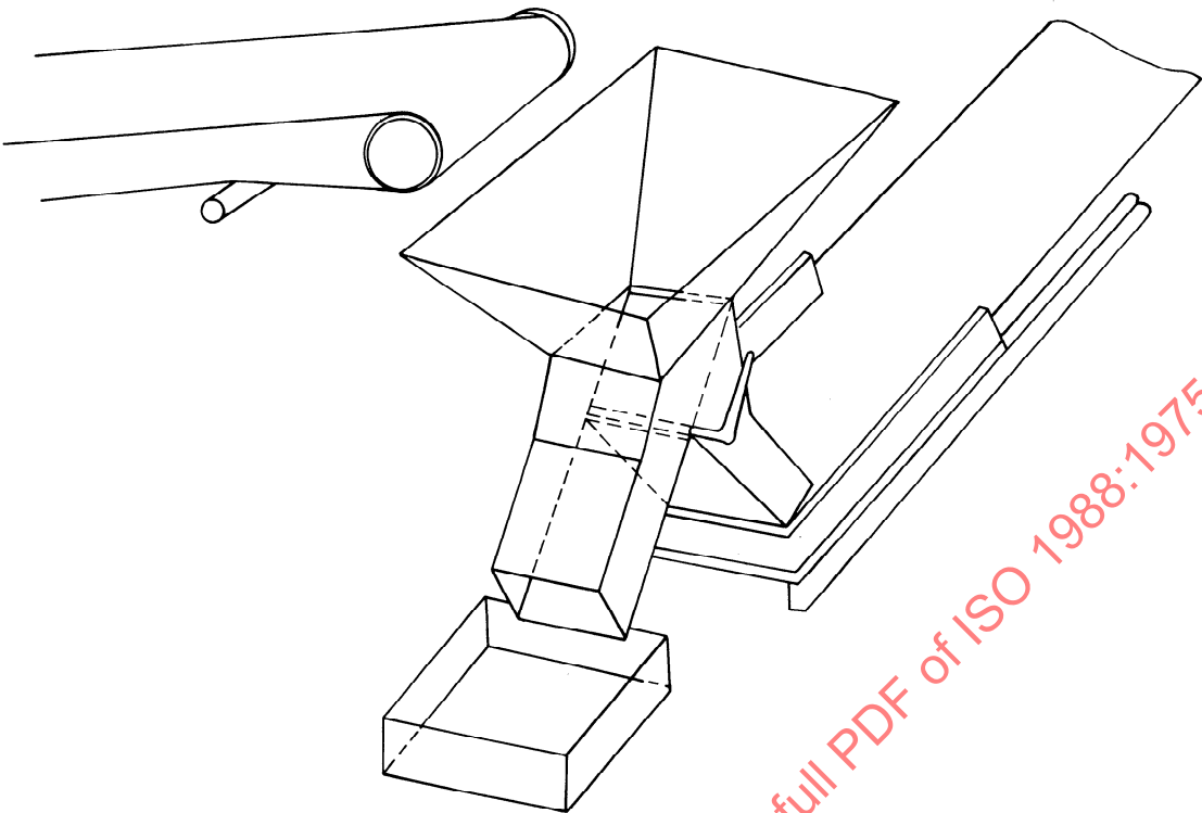
FIGURE 12 — Falling stream — Breeches chute
