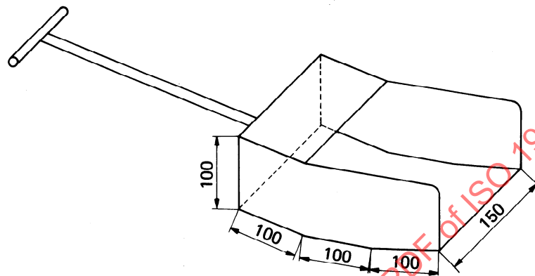
FIGURE 9 — Scoop (suitably dimensioned for coal of 50 mm top size)
