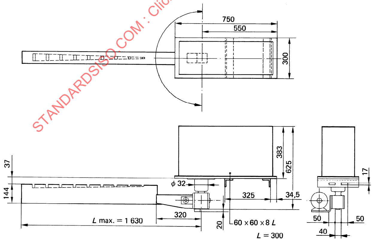
FIGURE 14 b) – Falling stream – Swinging arm
