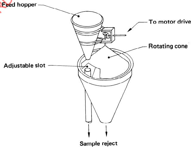
FIGURE 20 a) — Double cone sampler divider
