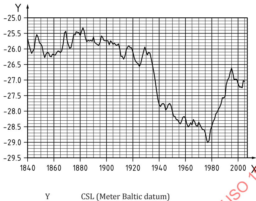
Figure F.3 — Long-term variation in Caspian Sea MSL
