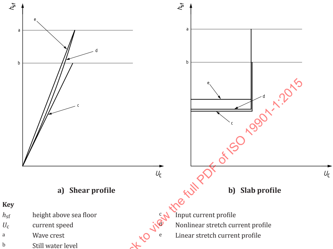
Figure A.5 — Linear and nonlinear stretching of current profiles
