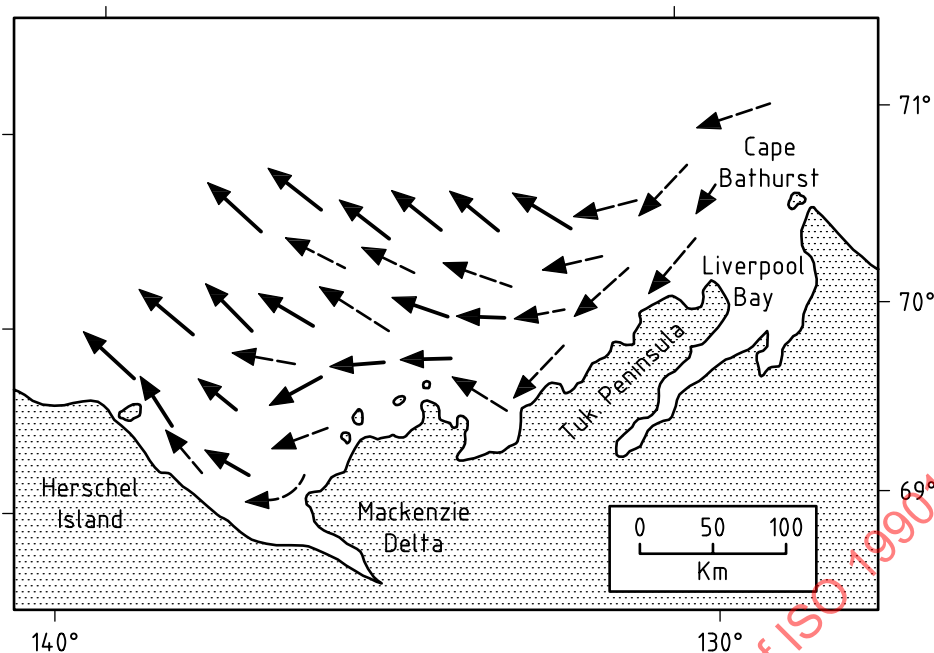
Figure D.6b — East winds
