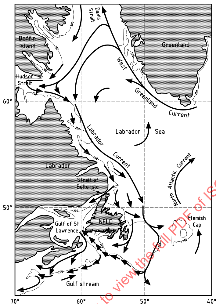
Figure D.3 — Canadian east coast ocean current regime
