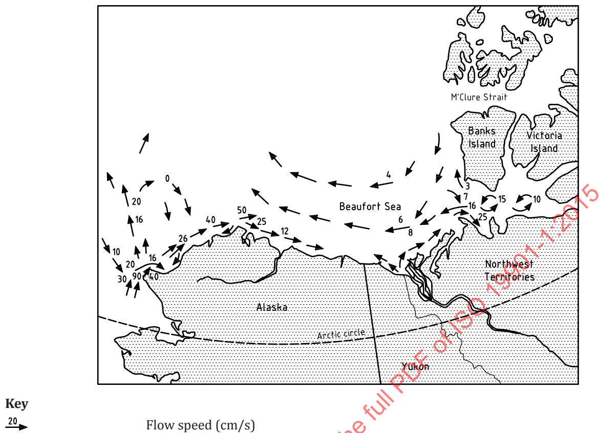
Figure D.5 — Mean general summer circulation of the surface water in the Beaufort and Chukchi Seas [173]
