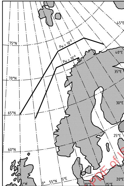
Figure B.3 — Limit of sea ice — Northwest Europe region — Annual probabilities of exceedance of 10^{-2} and 10^{-4}
