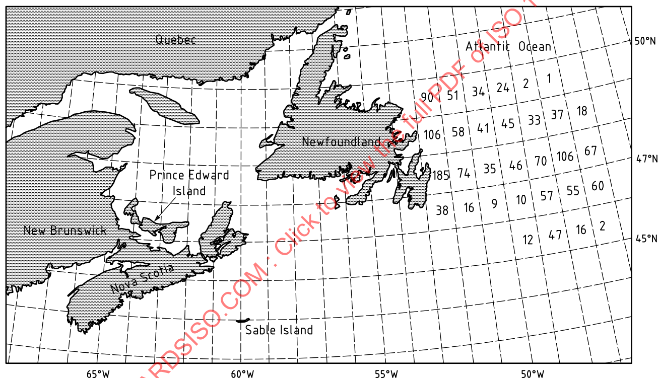
Figure D.12 — Historical yearly mean iceberg distribution offshore Newfoundland, based on data from 1981 to 2003 [176]
