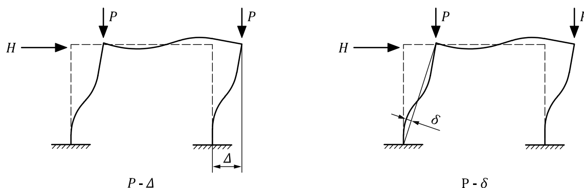
Figure A.7 — P-\Delta and P-\delta second order effects
