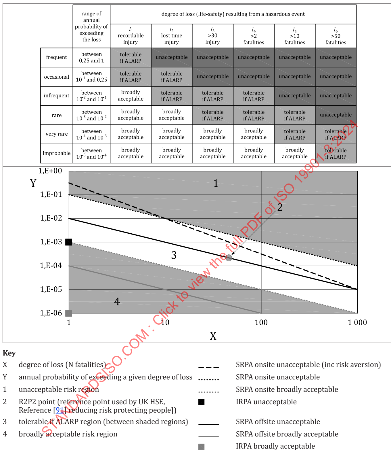
Figure 5 — Example risk matrix and example risk curve (based on UK HSE terminology and limits)
