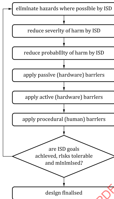
Figure A.1 — ISD and barrier steps for risk-based design
