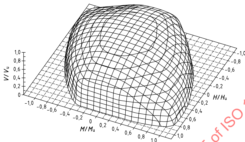
Figure A.4 — Yield surface for undrained conditions for a surface foundation with unlimited-uplift capacity along the foundation-soil interface[A.7-15]
