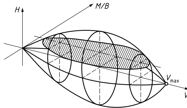
Figure A.6 — Yield surface for drained conditions for a surface foundation [A.7-28]
