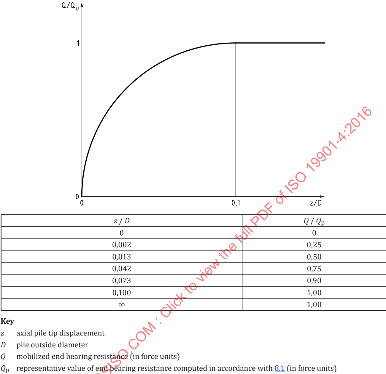
Figure 4— Typical pile end bearing resistance–displacement Q – z curve
