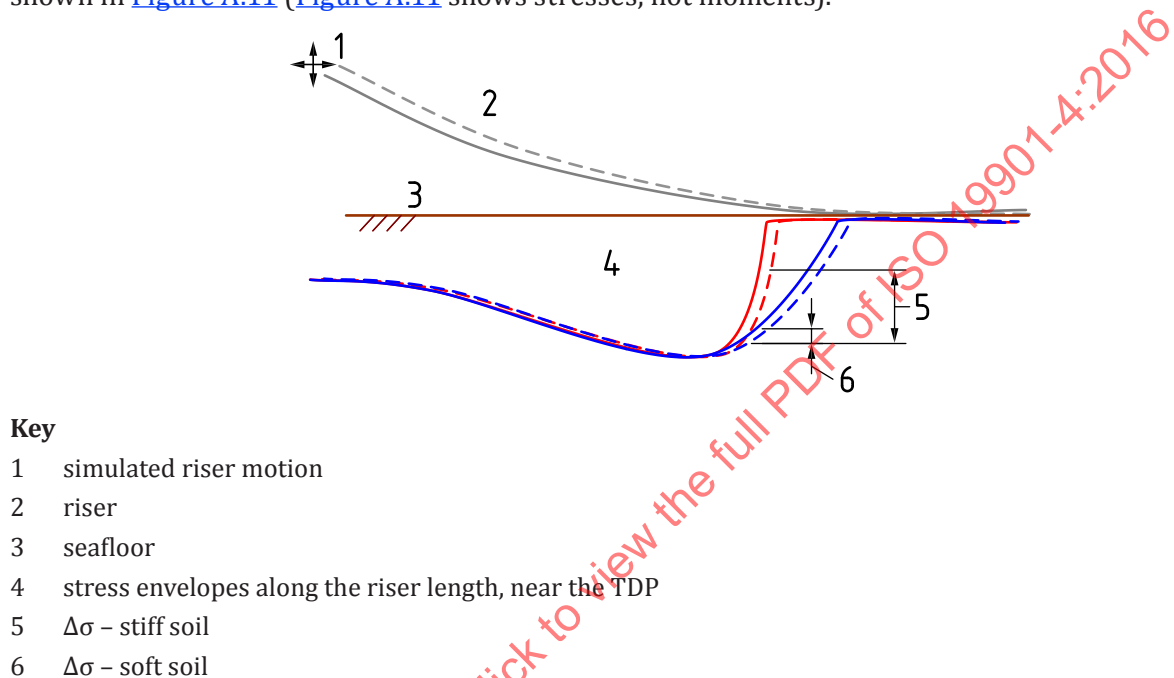
Figure A.11 — Example stress changes for fatigue calculations [A.10-1]
