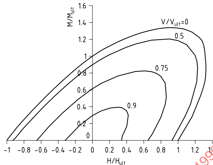
Figure A.5 — Yield surface for undrained conditions for an embedded foundation [A.7-19]
