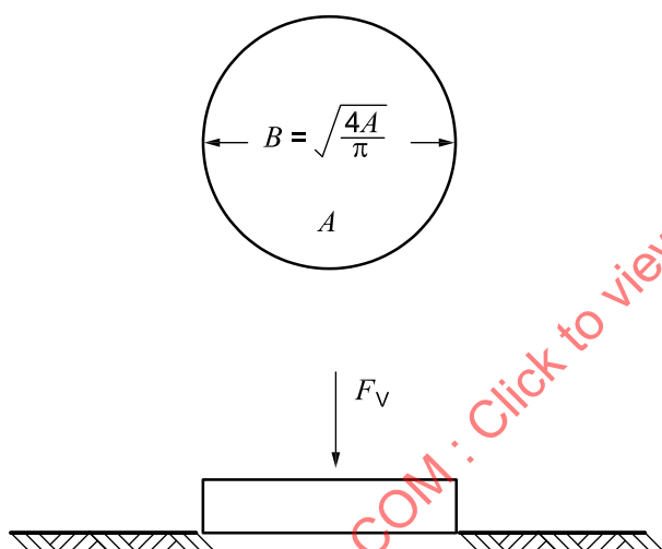
c) Equivalent model — Partially embedded
