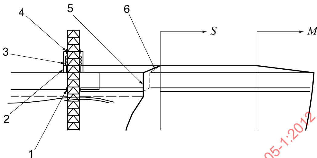
a) Jack-ups with a fixation system
