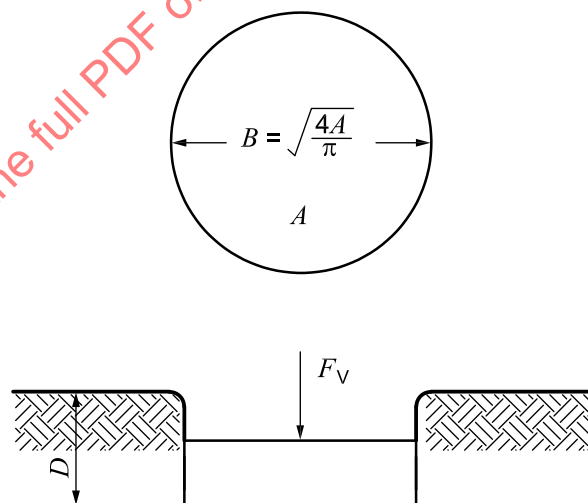
d) Equivalent model — Fully embedded
