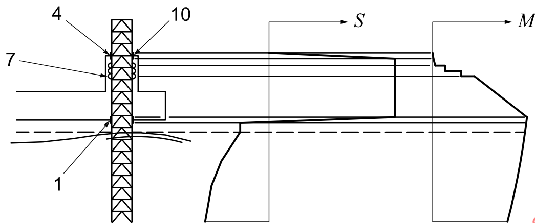
d) Jack-ups without a fixation system and having a floating jacking system
