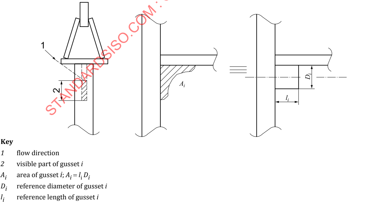
Figure A.7.3-2 — Gusset plates: equivalent modelling
