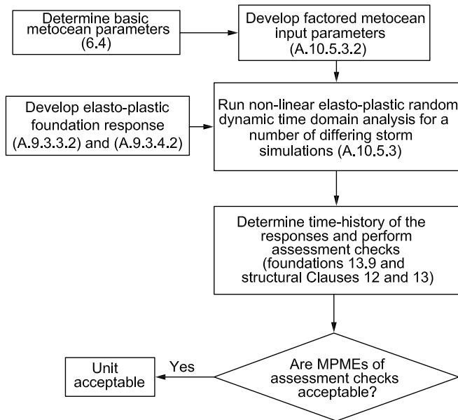
Figure A.10.5-4 — Analysis procedure for one-stage assessment with foundation fixity — Option 2
