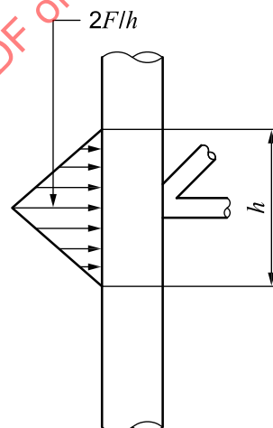
ii) Simplified distribution of the guide reaction
