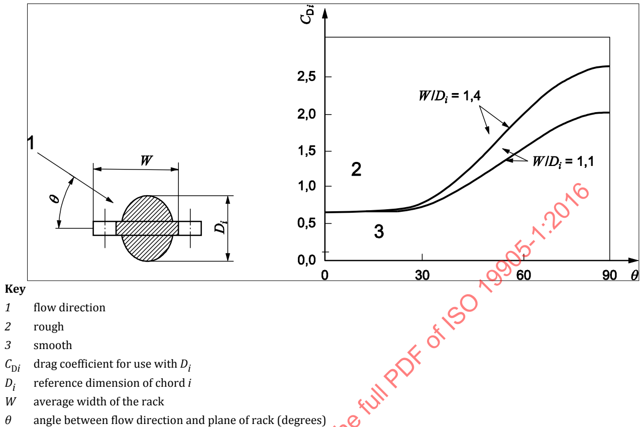
Figure A.7.3-3 — Split tube chord and typical values for C_{Di}
