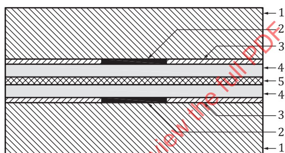
a) Configuration of test apparatus (Measurement A)
