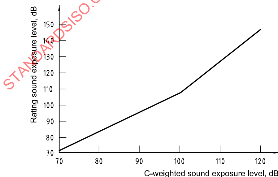
Figure B.1 — Rating sound exposure level as a function of C-weighted sound exposure level for high-energy impulse sounds
