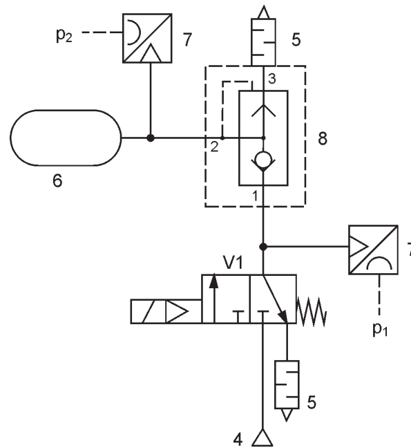
Figure 3 — Basic test equipment requirements for quick-exhaust valves
