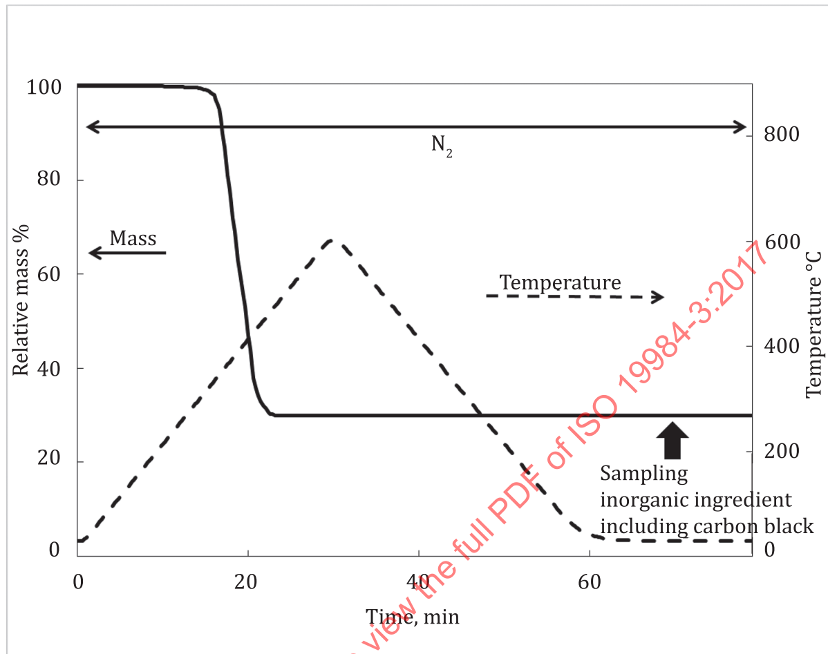
Figure 2 — Thermogram of thermogravimetric balance
