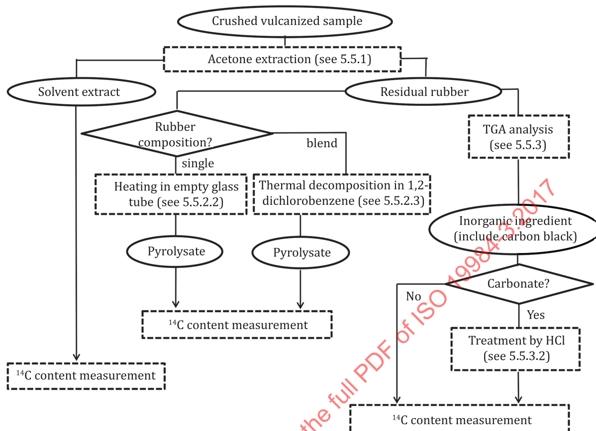
Figure 1 — Scheme of separating a vulcanized rubber to obtain a test sample for ^{14}\text{C} measurement
