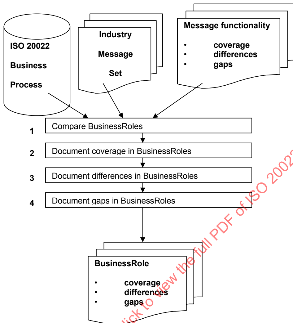
Figure 7 — Recommended approach for BusinessRoles gap analysis
