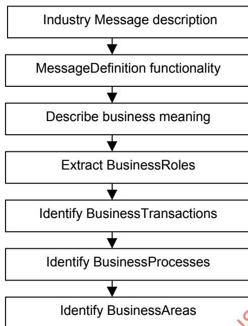
Figure 2 — Recommended approach to complete the IndustryMessageSet documentation
