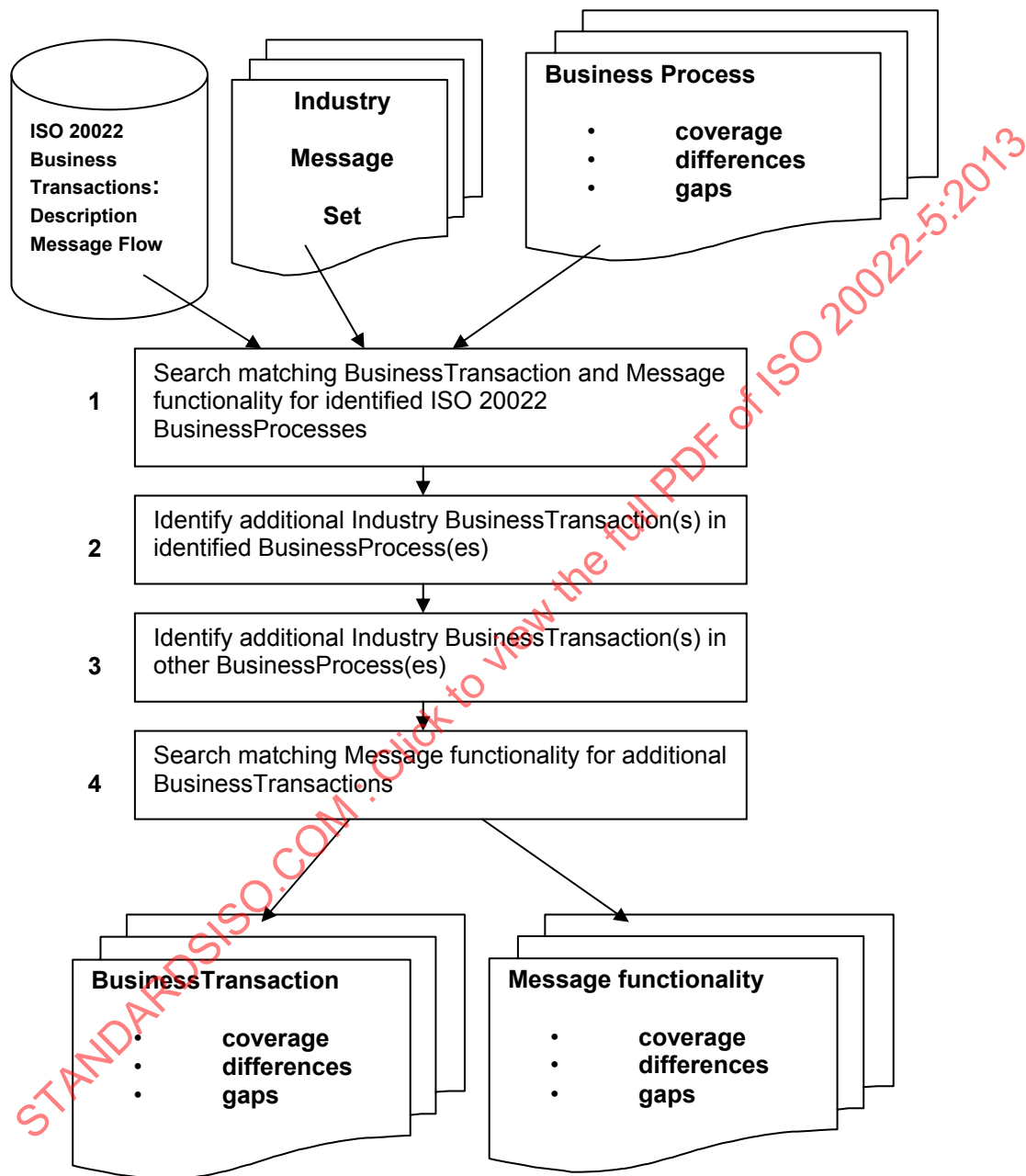
Figure 5 — Recommended approach for BusinessTransaction gap analysis
