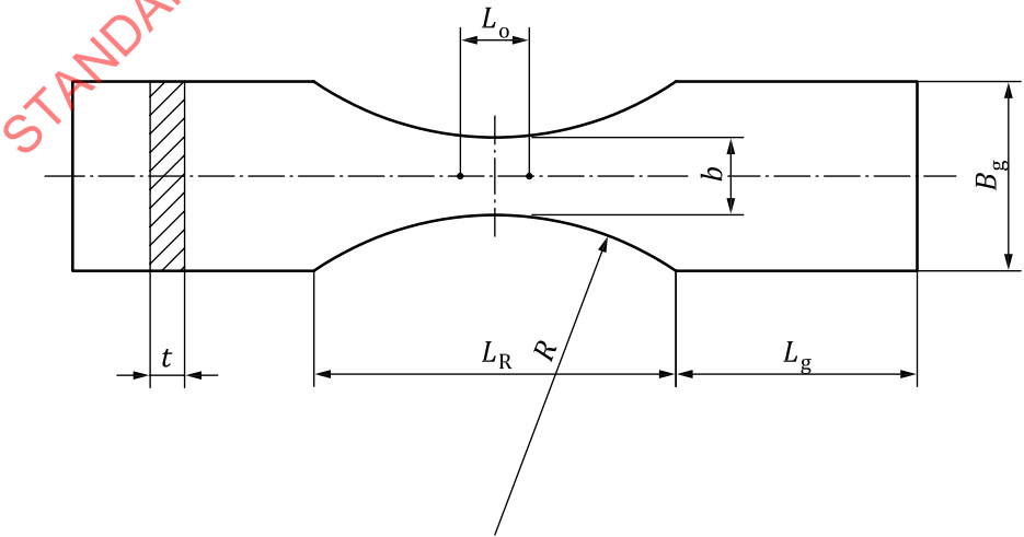
Figure 2 — Shape of R-type test piece
