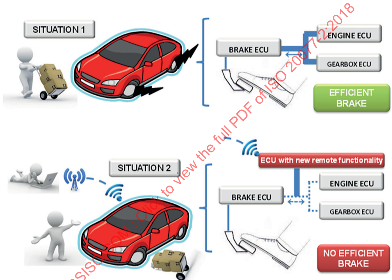
Figure 8 — Example of a potential safety related risk addressed by BP_008
