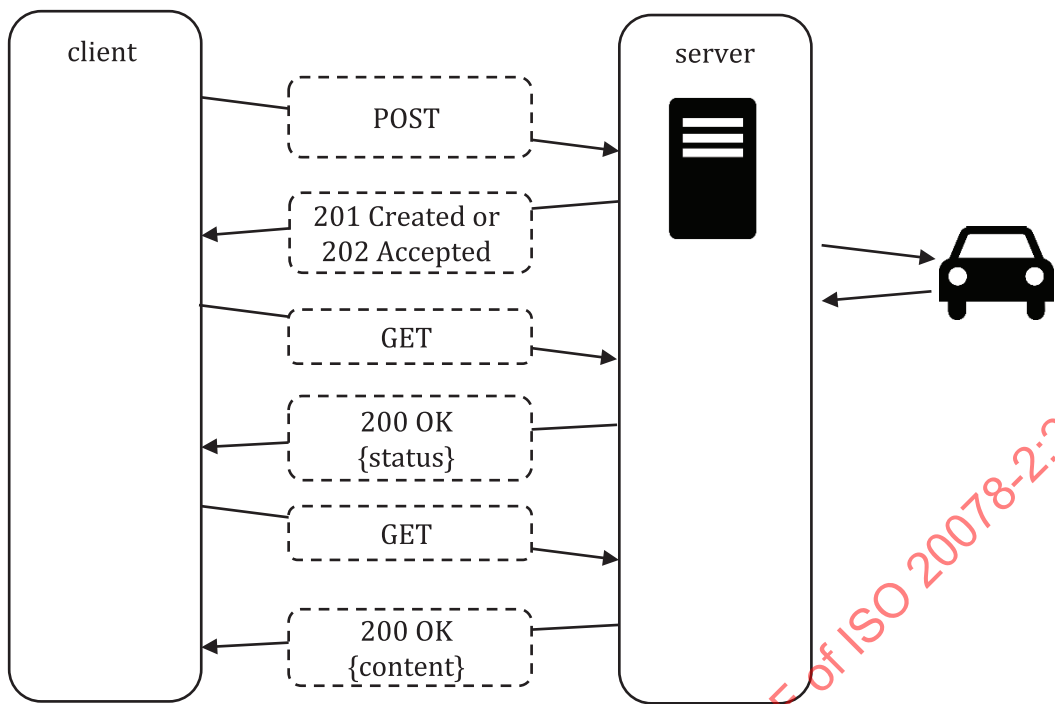
Figure 6 — Asynchronous interaction pattern
