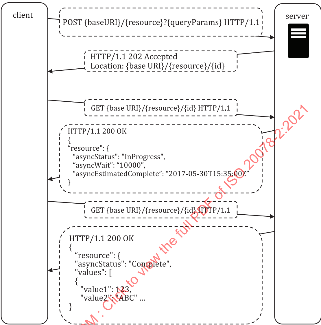
Figure 7 — Example of an asynchronous client server interaction
